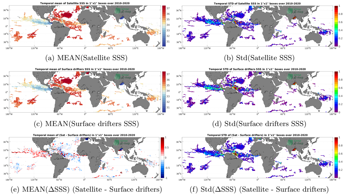
Figure 5: Temporal mean (left) and Std (right) of SSS from SMOS SSS L3 v335 - Monthly - 25 km (CATDS-CPDC) (top), Surface drifters (middle), and of \Delta SSS (Satellite - Surface drifters). Only match-up pairs are used to generate these maps.
