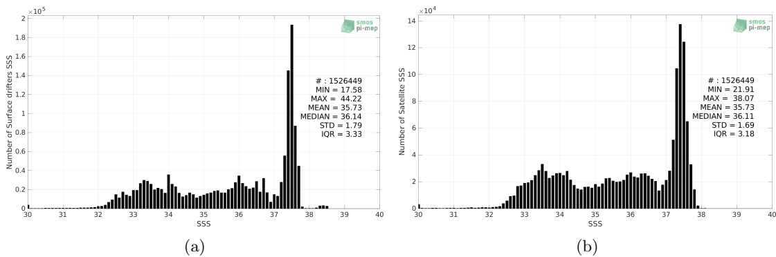
Figure 2: Histograms of SSS from Surface drifters (a) and SMOS SSS L3 v335 - Monthly - 25 km (CATDS-CPDC) (b) considering all match-up pairs per bins of 0.1 over the Mid-Low Latitudes 45N-45S Pi-MEP region and for the full satellite product period.
