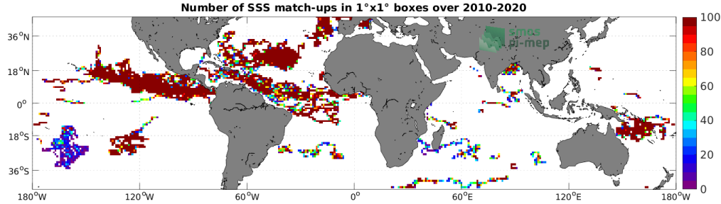
Figure 3: Number of SSS match-ups between Surface drifters SSS and the SMOS SSS L3 v335 - Monthly - 25 km (CATDS-CPDC) SSS product for the Mid-Low Latitudes 45N-45S Pi-MEP region over 1^\circ \times 1^\circ boxes and for the full satellite product period.
