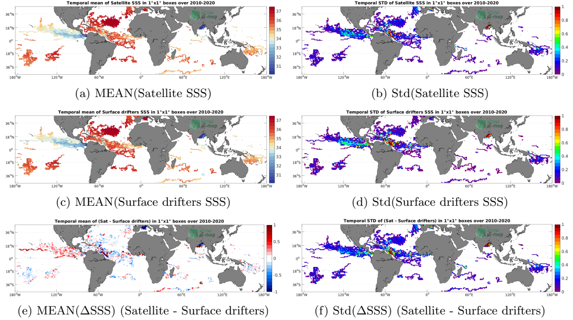
Figure 5: Temporal mean (left) and Std (right) of SSS from SMOS SSS L3 v335 - Monthly - 25 km (CATDS-CPDC) (top), Surface drifters (middle), and of \Delta\text{SSS} (Satellite - Surface drifters). Only match-up pairs are used to generate these maps.
