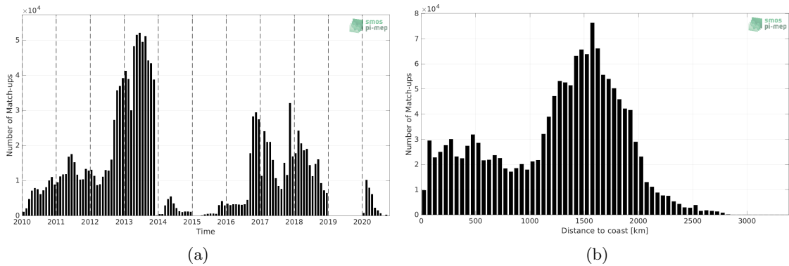
Figure 1: Number of match-ups between Surface drifters and SMOS SSS L3 v335 - Monthly - 25 km (CATDS-CPDC) SSS as a function of time (a) and as function of the distance to coast (b) over the Mid-Low Latitudes 45N-45S Pi-MEP region and for the full satellite product period.
