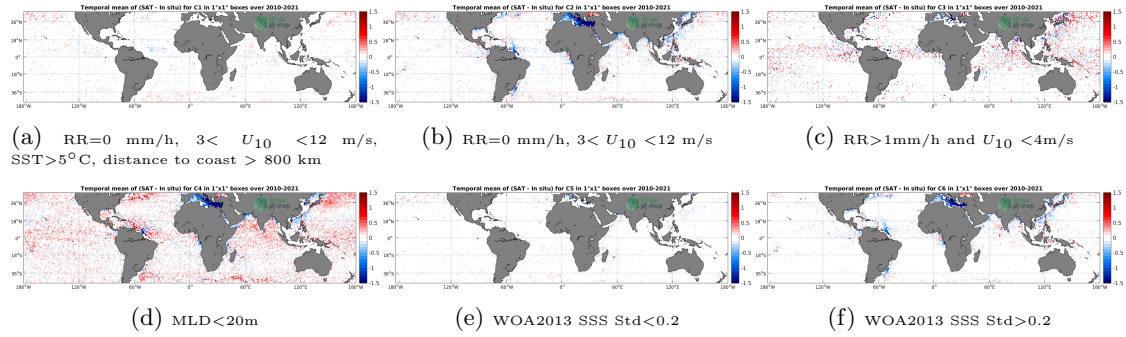
Figure 12: Temporal mean gridded over spatial boxes of size 1^\circ \times 1^\circ of \Delta SSS (SMOS SSS L3 v335 - Monthly - 25 km (CATDS-CPDC) - Argo) for 6 different subdatasets corresponding to: RR=0 mm/h, 3 < U_{10} < 12 m/s, SST > 5^\circ C , distance to coast > 800 km (a), RR=0 mm/h, 3 < U_{10} < 12 m/s (b), RR > 1 mm/h and U_{10} < 4 m/s (c), MLD < 20 m (d), WOA2013 SSS Std < 0.2 (e), WOA2013 SSS Std > 0.2 (f).
