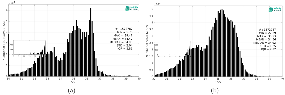
Figure 3: Histograms of SSS from TSG (SAMOS) (a) and SMOS SSS L3 v335 - 10 Days - 25 km (CATDS-CPDC) (b) considering all match-up pairs per bins of 0.1 over the Mid-Low Latitudes 45N-45S Pi-MEP region and for the full satellite product period.
