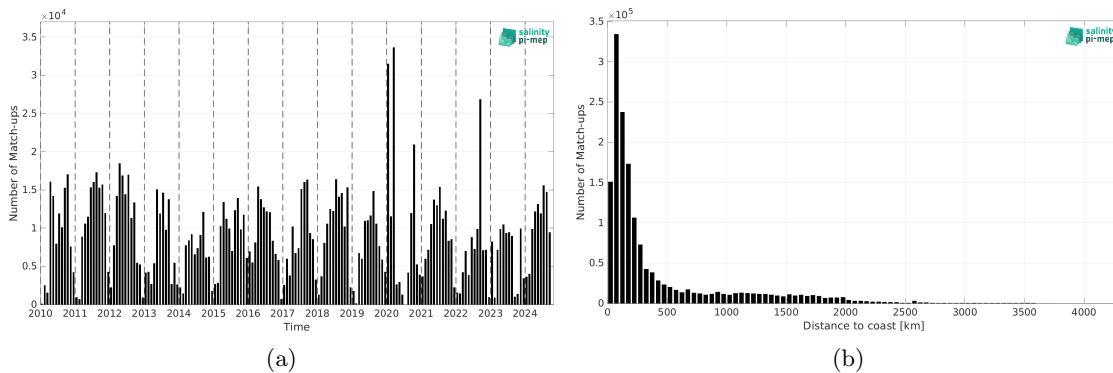
Figure 2: Number of match-ups between TSG (SAMOS) and SMOS SSS L3 v335 - 10 Days - 25 km (CATDS-CPDC) SSS as a function of time (a) and as function of the distance to coast (b) over the Mid-Low Latitudes 45N-45S Pi-MEP region and for the full satellite product period.
