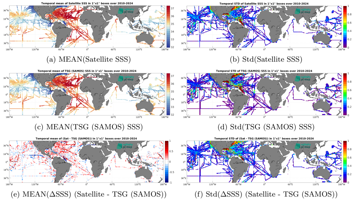
Figure 7: Temporal mean (left) and Std (right) of SSS from SMOS SSS L3 v335 - 10 Days - 25 km (CATDS-CPDC) (top), TSG (SAMOS) (middle), and of \Delta SSS (Satellite - TSG (SAMOS)). Only match-up pairs are used to generate these maps.
