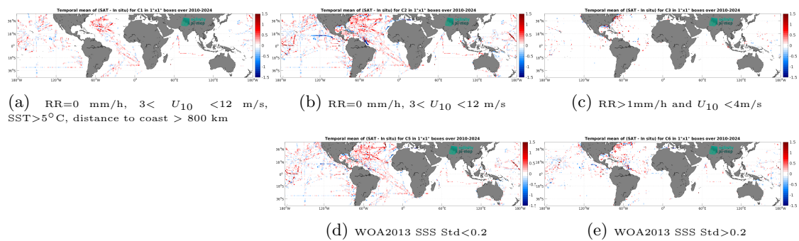
Figure 14: Temporal mean gridded over spatial boxes of size 1^\circ \times 1^\circ of \Delta\text{SSS} (SMOS SSS L3 v335 - 10 Days - 25 km (CATDS-CPDC) - TSG (SAMOS)) for 5 different subdatasets corresponding to:RR=0 mm/h, 3 < U_{10} < 12 m/s, SST > 5°C, distance to coast > 800 km (a), RR=0 mm/h, 3 < U_{10} < 12 m/s (b), RR > 1mm/h and U_{10} < 4 m/s (c), WOA2013 SSS Std < 0.2 (d), WOA2013 SSS Std > 0.2 (e).
