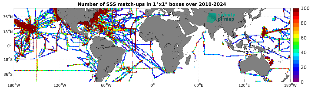
Figure 5: Number of SSS match-ups between TSG (SAMOS) SSS and the SMOS SSS L3 v335 - 10 Days - 25 km (CATDS-CPDC) SSS product for the Mid-Low Latitudes 45N-45S Pi-MEP region over 1^\circ \times 1^\circ boxes and for the full satellite product period.
