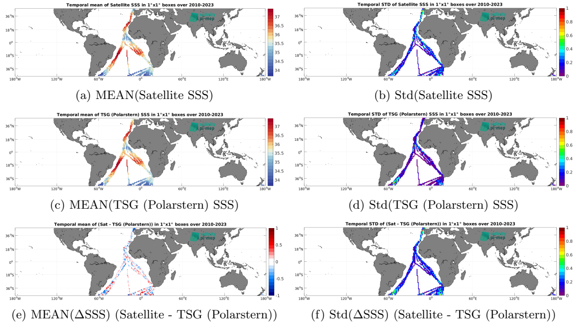
Figure 7: Temporal mean (left) and Std (right) of SSS from SMOS SSS L3 v335 - 10 Days - 25 km (CATDS-CPDC) (top), TSG (Polarstern) (middle), and of \Delta SSS (Satellite - TSG (Polarstern)). Only match-up pairs are used to generate these maps.
