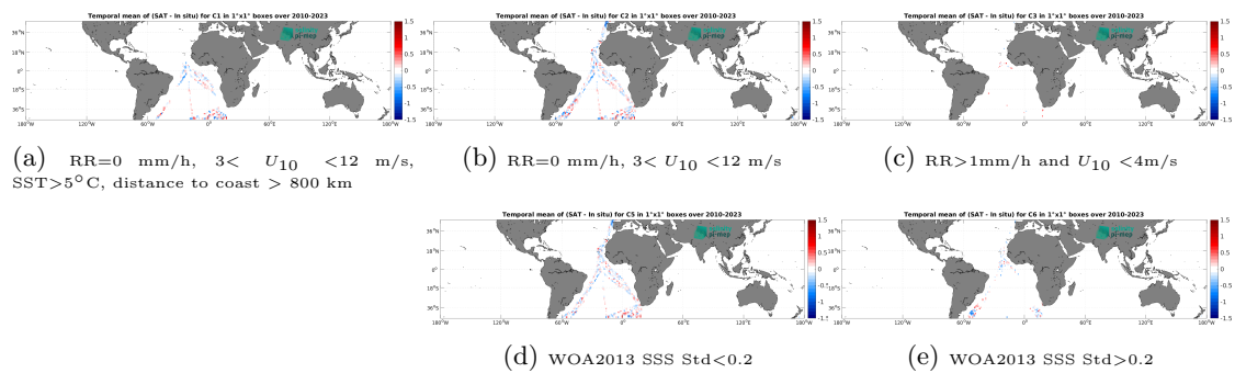
Figure 14: Temporal mean gridded over spatial boxes of size 1^\circ \times 1^\circ of \Delta\text{SSS} (SMOS SSS L3 v335 - 10 Days - 25 km (CATDS-CPDC) - TSG (Polarstern)) for 5 different subdatasets corresponding to: RR=0 mm/h, 3 < U_{10} < 12 m/s, SST > 5°C, distance to coast > 800 km (a), RR=0 mm/h, 3 < U_{10} < 12 m/s (b), RR > 1mm/h and U_{10} < 4 m/s (c), WOA2013 SSS Std < 0.2 (d), WOA2013 SSS Std > 0.2 (e).
