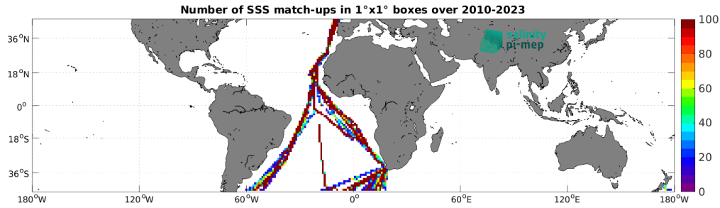
Figure 5: Number of SSS match-ups between TSG (Polarstern) SSS and the SMOS SSS L3 v335 - 10 Days - 25 km (CATDS-CPDC) SSS product for the Mid-Low Latitudes 45N-45S Pi-MEP region over 1^\circ \times 1^\circ boxes and for the full satellite product period.
