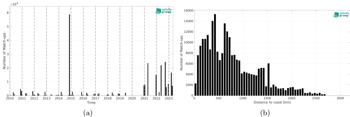
Figure 2: Number of match-ups between TSG (Polarstern) and SMOS SSS L3 v335 - 10 Days - 25 km (CATDS-CPDC) SSS as a function of time (a) and as function of the distance to coast (b) over the Mid-Low Latitudes 45N-45S Pi-MEP region and for the full satellite product period.
