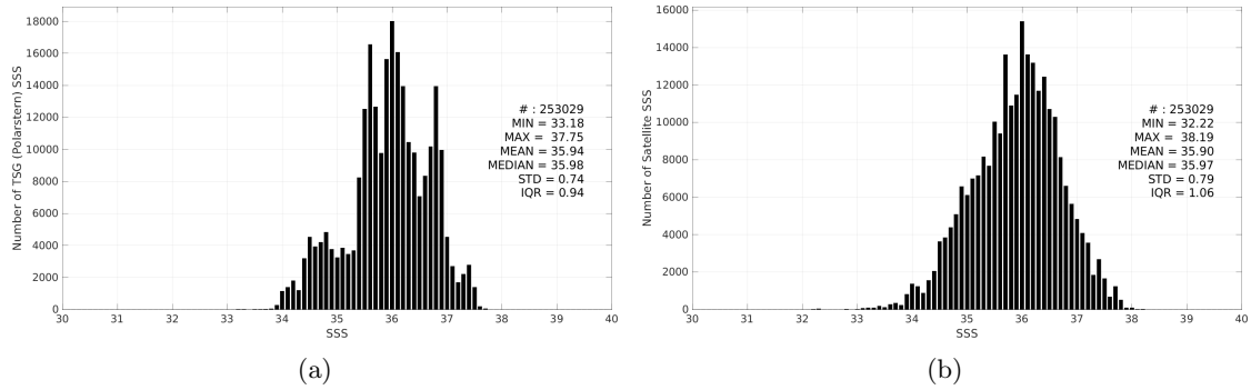
Figure 3: Histograms of SSS from TSG (Polarstern) (a) and SMOS SSS L3 v335 - 10 Days - 25 km (CATDS-CPDC) (b) considering all match-up pairs per bins of 0.1 over the Mid-Low Latitudes 45N-45S Pi-MEP region and for the full satellite product period.
