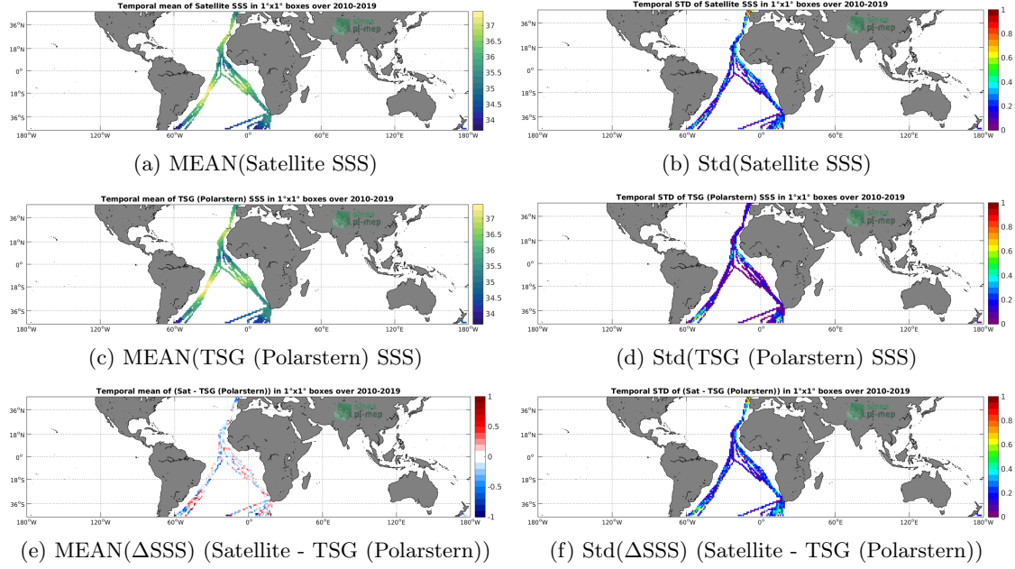
Figure 6: Temporal mean (left) and Std (right) of SSS from SMOS SSS L3 v335 - 10 Days - 25 km (CATDS-CPDC) (top), TSG (Polarstern) (middle), and of \Delta SSS (Satellite - TSG (Polarstern)). Only match-up pairs are used to generate these maps.
