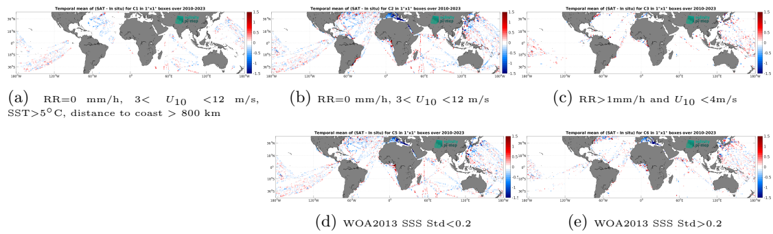
Figure 14: Temporal mean gridded over spatial boxes of size 1^\circ \times 1^\circ of \Delta\text{SSS} (SMOS SSS L3 v335 - 10 Days - 25 km (CATDS-CPDC) - TSG (LEGOS-DM)) for 5 different subdatasets corresponding to: RR=0 mm/h, 3 < U_{10} < 12 m/s, SST > 5°C, distance to coast > 800 km (a), RR=0 mm/h, 3 < U_{10} < 12 m/s (b), RR > 1mm/h and U_{10} < 4 m/s (c), WOA2013 SSS Std < 0.2 (d), WOA2013 SSS Std > 0.2 (e).
