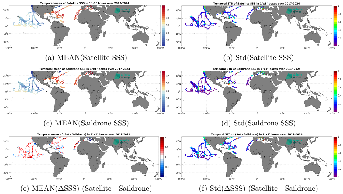
Figure 7: Temporal mean (left) and Std (right) of SSS from SMOS SSS L3 v335 - 10 Days - 25 km (CATDS-CPDC) (top), Saildrone (middle), and of \Delta SSS (Satellite - Saildrone). Only match-up pairs are used to generate these maps.
