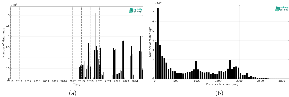
Figure 2: Number of match-ups between Saildrone and SMOS SSS L3 v335 - 10 Days - 25 km (CATDS-CPDC) SSS as a function of time (a) and as function of the distance to coast (b) over the Mid-Low Latitudes 45N-45S Pi-MEP region and for the full satellite product period.
