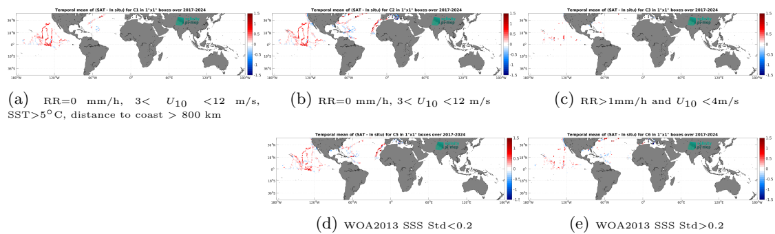
Figure 14: Temporal mean gridded over spatial boxes of size 1^\circ \times 1^\circ of \Delta\text{SSS} (SMOS SSS L3 v335 - 10 Days - 25 km (CATDS-CPDC) - Saildrone) for 5 different subdatasets corresponding to: RR=0 mm/h, 3 < U_{10} < 12 m/s, SST > 5°C, distance to coast > 800 km (a), RR=0 mm/h, 3 < U_{10} < 12 m/s (b), RR > 1mm/h and U_{10} < 4 m/s (c), WOA2013 SSS Std < 0.2 (d), WOA2013 SSS Std > 0.2 (e).
