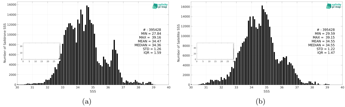
Figure 3: Histograms of SSS from Saildrone (a) and SMOS SSS L3 v335 - 10 Days - 25 km (CATDS-CPDC) (b) considering all match-up pairs per bins of 0.1 over the Mid-Low Latitudes 45N-45S Pi-MEP region and for the full satellite product period.
