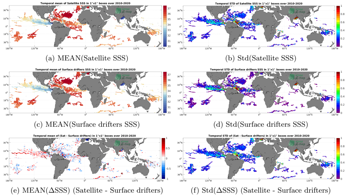
Figure 5: Temporal mean (left) and Std (right) of SSS from SMOS SSS L3 v335 - 10 Days - 25 km (CATDS-CPDC) (top), Surface drifters (middle), and of \Delta SSS (Satellite - Surface drifters). Only match-up pairs are used to generate these maps.
