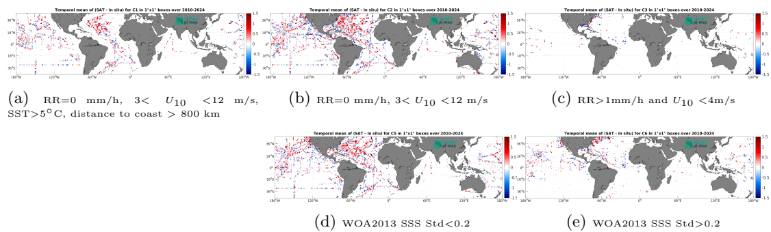
Figure 14: Temporal mean gridded over spatial boxes of size 1^\circ \times 1^\circ of \Delta\text{SSS} (SMOS SSS L2Q v333 - 0.25 Deg (CATDS-CPDC) - TSG (SAMOS)) for 5 different subdatasets corresponding to: RR=0 mm/h, 3 < U_{10} < 12 m/s, SST>5°C, distance to coast > 800 km (a), RR=0 mm/h, 3 < U_{10} < 12 m/s (b), RR>1mm/h and U_{10} < 4 m/s (c), WOA2013 SSS Std<0.2 (d), WOA2013 SSS Std>0.2 (e).
