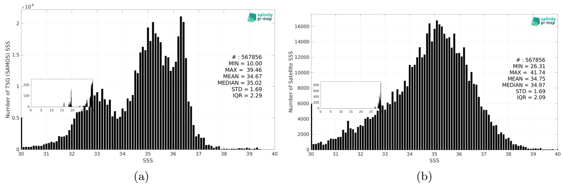
Figure 3: Histograms of SSS from TSG (SAMOS) (a) and SMOS SSS L2Q v333 - 0.25 Deg (CATDS-CPDC) (b) considering all match-up pairs per bins of 0.1 over the Mid-Low Latitudes 45N-45S Pi-MEP region and for the full satellite product period.
