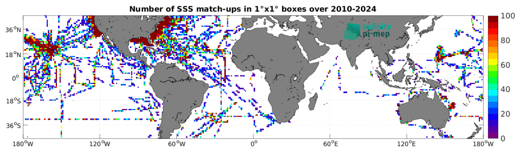
Figure 5: Number of SSS match-ups between TSG (SAMOS) SSS and the SMOS SSS L2Q v333 - 0.25 Deg (CATDS-CPDC) SSS product for the Mid-Low Latitudes 45N-45S Pi-MEP region over 1^\circ \times 1^\circ boxes and for the full satellite product period.
