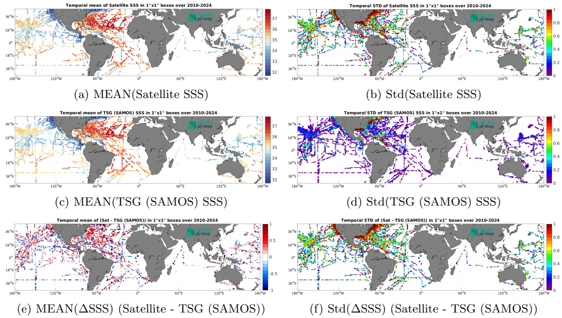
Figure 7: Temporal mean (left) and Std (right) of SSS from SMOS SSS L2Q v333 - 0.25 Deg (CATDS-CPDC) (top), TSG (SAMOS) (middle), and of \Delta SSS (Satellite - TSG (SAMOS)). Only match-up pairs are used to generate these maps.
