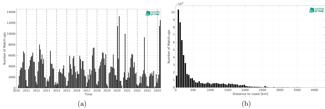
Figure 2: Number of match-ups between TSG (SAMOS) and SMOS SSS L2Q v333 - 0.25 Deg (CATDS-CPDC) SSS as a function of time (a) and as function of the distance to coast (b) over the Mid-Low Latitudes 45N-45S Pi-MEP region and for the full satellite product period.
