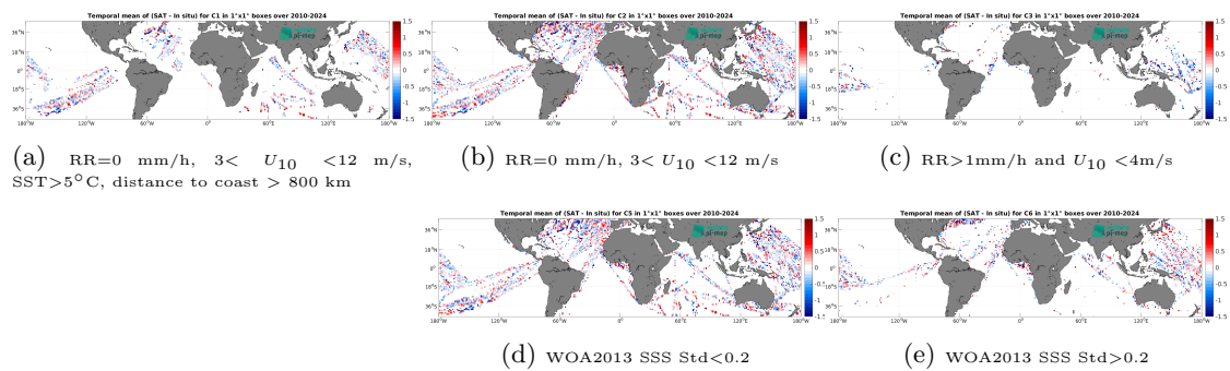
Figure 14: Temporal mean gridded over spatial boxes of size 1^\circ \times 1^\circ of \Delta SSS (SMOS SSS L2Q v333 - 0.25 Deg (CATDS-CPDC) - TSG (LEGOS-DM)) for 5 different subdatasets corresponding to: RR=0 mm/h, 3 < U_{10} < 12 m/s, SST > 5^\circ\text{C} , distance to coast > 800 km (a), RR=0 mm/h, 3 < U_{10} < 12 m/s (b), RR > 1 mm/h and U_{10} < 4 m/s (c), WOA2013 SSS Std < 0.2 (d), WOA2013 SSS Std > 0.2 (e).
