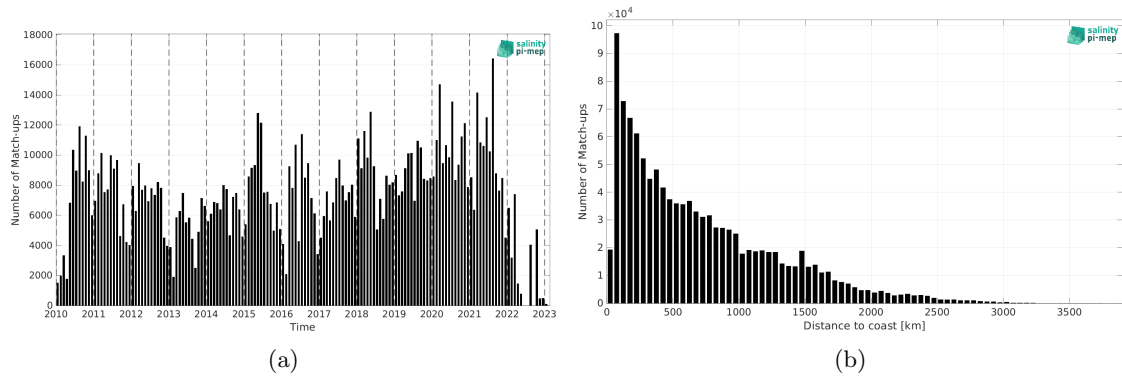
Figure 2: Number of match-ups between TSG (LEGOS-DM) and SMOS SSS L2Q v333 - 0.25 Deg (CATDS-CPDC) SSS as a function of time (a) and as function of the distance to coast (b) over the Mid-Low Latitudes 45N-45S Pi-MEP region and for the full satellite product period.
