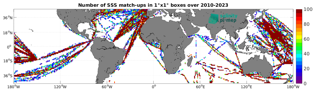
Figure 5: Number of SSS match-ups between TSG (LEGOS-DM) SSS and the SMOS SSS L2Q v333 - 0.25 Deg (CATDS-CPDC) SSS product for the Mid-Low Latitudes 45N-45S Pi-MEP region over 1^\circ \times 1^\circ boxes and for the full satellite product period.
