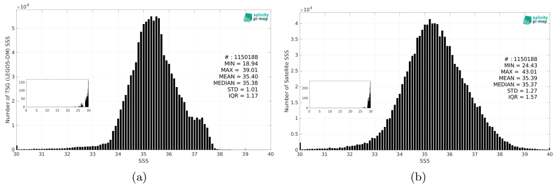
Figure 3: Histograms of SSS from TSG (LEGOS-DM) (a) and SMOS SSS L2Q v333 - 0.25 Deg (CATDS-CPDC) (b) considering all match-up pairs per bins of 0.1 over the Mid-Low Latitudes 45N-45S Pi-MEP region and for the full satellite product period.
