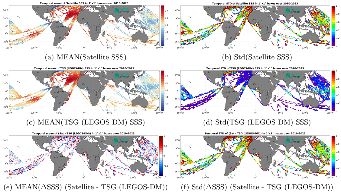
Figure 7: Temporal mean (left) and Std (right) of SSS from SMOS SSS L2Q v333 - 0.25 Deg (CATDS-CPDC) (top), TSG (LEGOS-DM) (middle), and of \Delta SSS (Satellite - TSG (LEGOS-DM)). Only match-up pairs are used to generate these maps.
