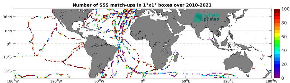
Figure 5: Number of SSS match-ups between TSG (GOSUD-Sailing-ship) SSS and the SMOS SSS L2Q v333 - 0.25 Deg (CATDS-CPDC) SSS product for the Mid-Low Latitudes 45N-45S Pi-MEP region over 1^\circ \times 1^\circ boxes and for the full satellite product period.
