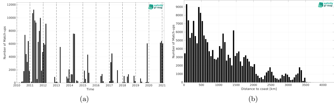
Figure 2: Number of match-ups between TSG (GOSUD-Sailing-ship) and SMOS SSS L2Q v333 - 0.25 Deg (CATDS-CPDC) SSS as a function of time (a) and as function of the distance to coast (b) over the Mid-Low Latitudes 45N-45S Pi-MEP region and for the full satellite product period.
