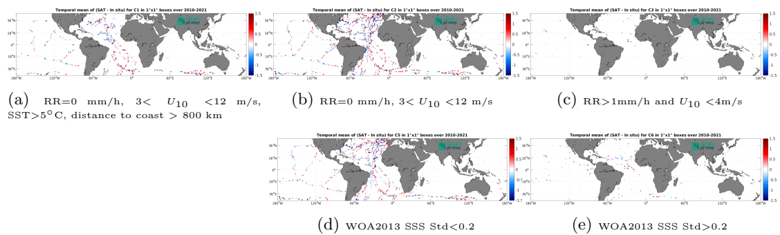
Figure 14: Temporal mean gridded over spatial boxes of size 1^\circ \times 1^\circ of \Delta\text{SSS} (SMOS SSS L2Q v333 - 0.25 Deg (CATDS-CPDC) - TSG (GOSUD-Sailing-ship)) for 5 different subdatasets corresponding to: RR=0 mm/h, 3 < U_{10} < 12 m/s, SST > 5°C, distance to coast > 800 km (a), RR=0 mm/h, 3 < U_{10} < 12 m/s (b), RR > 1mm/h and U_{10} < 4 m/s (c), WOA2013 SSS Std < 0.2 (d), WOA2013 SSS Std > 0.2 (e).
