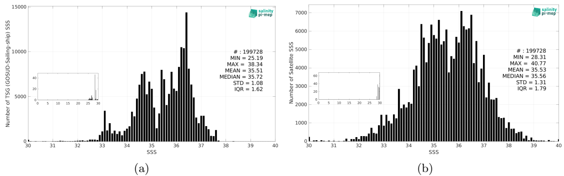
Figure 3: Histograms of SSS from TSG (GOSUD-Sailing-ship) (a) and SMOS SSS L2Q v333 - 0.25 Deg (CATDS-CPDC) (b) considering all match-up pairs per bins of 0.1 over the Mid-Low Latitudes 45N-45S Pi-MEP region and for the full satellite product period.
