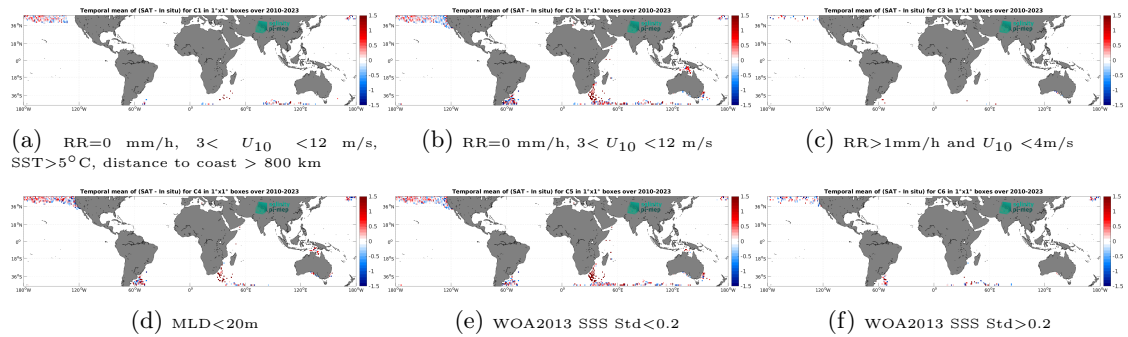
Figure 14: Temporal mean gridded over spatial boxes of size 1^\circ \times 1^\circ of \Delta SSS (SMOS SSS L2Q v333 - 0.25 Deg (CATDS-CPDC) - Marine mammals) for 6 different subdatasets corresponding to:RR=0 mm/h, 3 < U_{10} < 12 m/s, SST >5^\circ C, distance to coast > 800 km (a), RR=0 mm/h, 3 < U_{10} < 12 m/s (b), RR >1 mm/h and U_{10} < 4 m/s (c),MLD <20 m (d),WOA2013 SSS Std <0.2 (e),WOA2013 SSS Std >0.2 (f).
