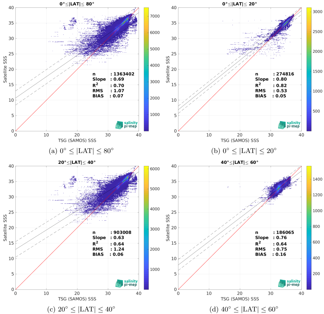
Figure 9: Contour maps of the concentration of SMOS SSS L3 v332 - 9 Days (CATDS-CPDC) SSS (y-axis) versus TSG (SAMOS) SSS (x-axis) at match-up pairs for different latitude bands. For each plot, the red line shows x=y . The black thin and dashed lines indicate a linear fit through the data cloud and the \pm 95\% confidence levels, respectively. The number match-up pairs n , the slope and R^2 coefficient of the linear fit, the root mean square (RMS) and the mean bias between satellite and in situ data are indicated for each latitude band in each plot.
