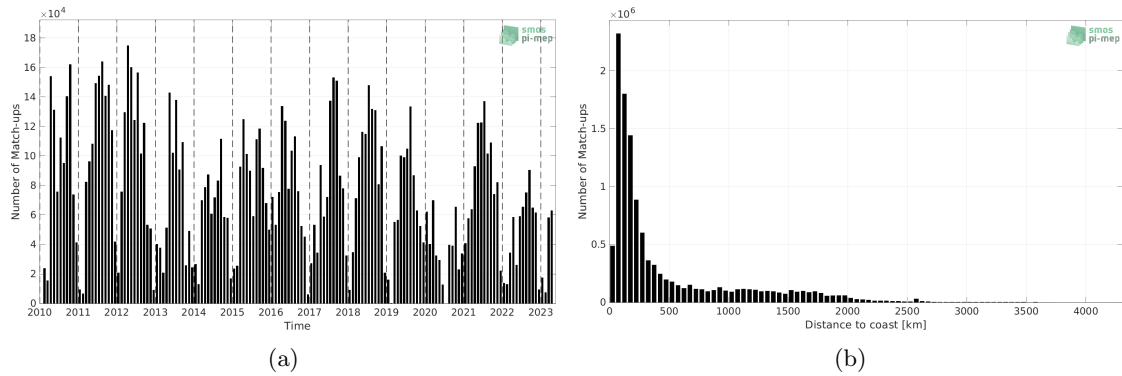
Figure 1: Number of match-ups between TSG (SAMOS) and SMOS SSS L3 v332 - 9 Days (CATDS-CPDC) SSS as a function of time (a) and as function of the distance to coast (b) over the Mid-Low Latitudes 45N-45S Pi-MEP region and for the full satellite product period.
