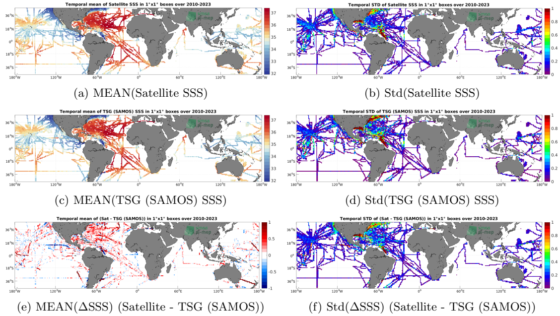
Figure 6: Temporal mean (left) and Std (right) of SSS from SMOS SSS L3 v332 - 9 Days (CATDS-CPDC) (top), TSG (SAMOS) (middle), and of \Delta SSS (Satellite - TSG (SAMOS)). Only match-up pairs are used to generate these maps.
