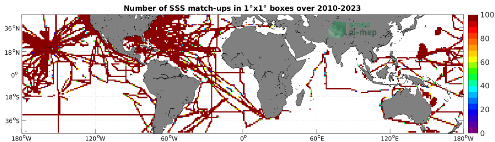
Figure 4: Number of SSS match-ups between TSG (SAMOS) SSS and the SMOS SSS L3 v332 - 9 Days (CATDS-CPDC) SSS product for the Mid-Low Latitudes 45N-45S Pi-MEP region over 1^\circ \times 1^\circ boxes and for the full satellite product period.
