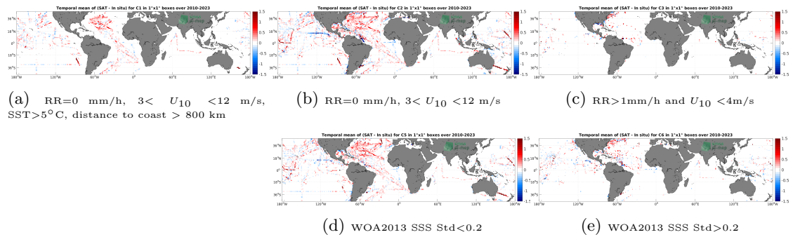
Figure 12: Temporal mean gridded over spatial boxes of size 1^\circ \times 1^\circ of \Delta SSS (SMOS SSS L3 v332 - 9 Days (CATDS-CPDC) - TSG (SAMOS)) for 5 different subdatasets corresponding to:RR=0 mm/h, 3 < U_{10} < 12 m/s, SST > 5^\circ\text{C} , distance to coast > 800 km (a), RR=0 mm/h, 3 < U_{10} < 12 m/s (b), RR > 1 mm/h and U_{10} < 4 m/s (c), WOA2013 SSS Std < 0.2 (d), WOA2013 SSS Std > 0.2 (e).
