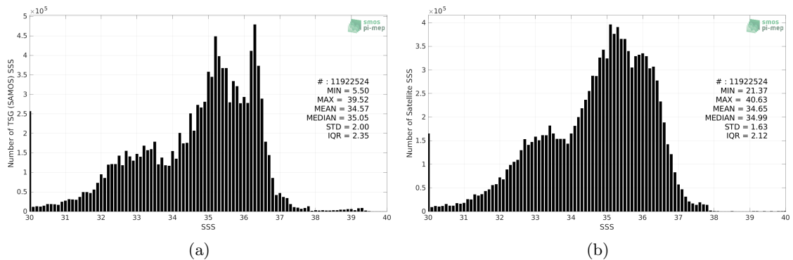
Figure 2: Histograms of SSS from TSG (SAMOS) (a) and SMOS SSS L3 v332 - 9 Days (CATDS-CPDC) (b) considering all match-up pairs per bins of 0.1 over the Mid-Low Latitudes 45N-45S Pi-MEP region and for the full satellite product period.
