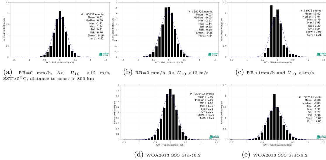
Figure 15: Normalized histogram of \Delta\text{SSS} (SMOS SSS L3 v332 - 9 Days (CATDS-CPDC) - TSG (Polarstern)) for 5 different subdatasets corresponding to: RR=0 mm/h, 3 < U_{10} < 12 m/s, SST>5°C, distance to coast > 800 km (a), RR=0 mm/h, 3 < U_{10} < 12 m/s (b), RR>1mm/h and U_{10} < 4 m/s (c), WOA2013 SSS Std<0.2 (d), WOA2013 SSS Std>0.2 (e).
