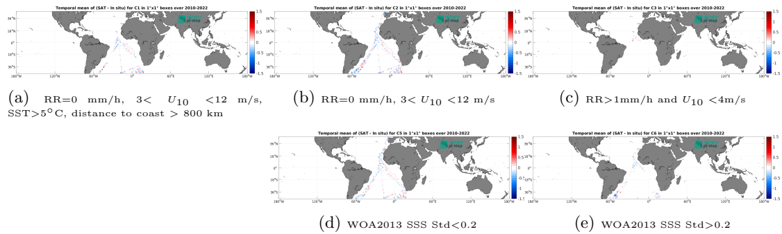
Figure 12: Temporal mean gridded over spatial boxes of size 1^\circ \times 1^\circ of \Delta\text{SSS} (SMOS SSS L3 v332 - 9 Days (CATDS-CPDC) - TSG (Polarstern)) for 5 different subdatasets corresponding to:RR=0 mm/h, 3 < U_{10} < 12 m/s, SST >5^\circ\text{C} , distance to coast > 800 km (a), RR=0 mm/h, 3 < U_{10} < 12 m/s (b), RR >1 mm/h and U_{10} < 4 m/s (c), WOA2013 SSS Std <0.2 (d), WOA2013 SSS Std >0.2 (e).
