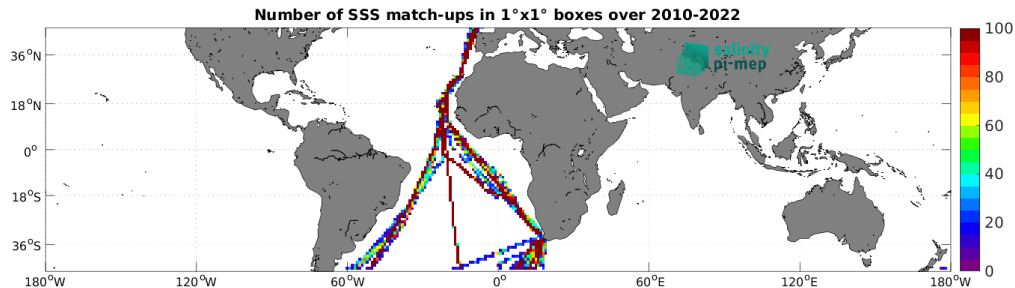
Figure 4: Number of SSS match-ups between TSG (Polarstern) SSS and the SMOS SSS L3 v332 - 9 Days (CATDS-CPDC) SSS product for the Mid-Low Latitudes 45N-45S Pi-MEP region over 1^\circ \times 1^\circ boxes and for the full satellite product period.
