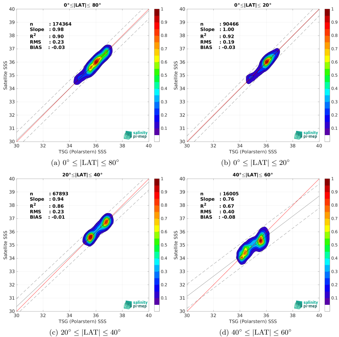
Figure 9: Contour maps of the concentration of SMOS SSS L3 v332 - 9 Days (CATDS-CPDC) SSS (y-axis) versus TSG (Polarstern) SSS (x-axis) at match-up pairs for different latitude bands. For each plot, the red line shows x=y . The black thin and dashed lines indicate a linear fit through the data cloud and the \pm 95\% confidence levels, respectively. The number match-up pairs n , the slope and R^2 coefficient of the linear fit, the root mean square (RMS) and the mean bias between satellite and in situ data are indicated for each latitude band in each plots.
