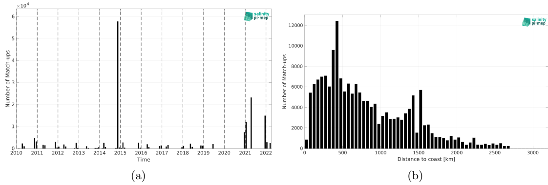
Figure 1: Number of match-ups between TSG (Polarstern) and SMOS SSS L3 v332 - 9 Days (CATDS-CPDC) SSS as a function of time (a) and as function of the distance to coast (b) over the Mid-Low Latitudes 45N-45S Pi-MEP region and for the full satellite product period.
