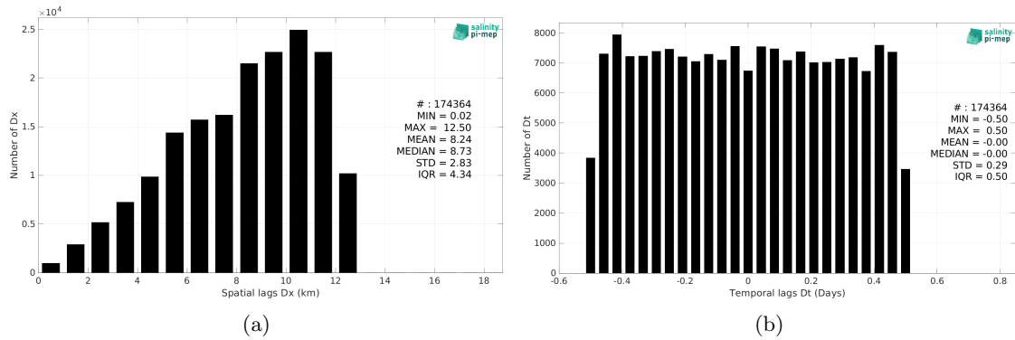
Figure 5: Histograms of the spatial (a) and temporal (b) lags between the location/time of the TSG (Polarstern) measurement and the date of the corresponding SMOS SSS L3 v332 - 9 Days (CATDS-CPDC) SSS pixel.
