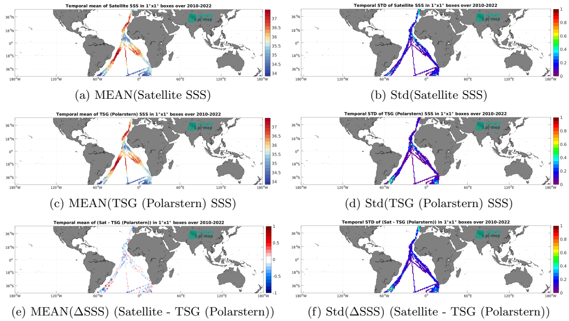
Figure 6: Temporal mean (left) and Std (right) of SSS from SMOS SSS L3 v332 - 9 Days (CATDS-CPDC) (top), TSG (Polarstern) (middle), and of \Delta SSS (Satellite - TSG (Polarstern)). Only match-up pairs are used to generate these maps.
