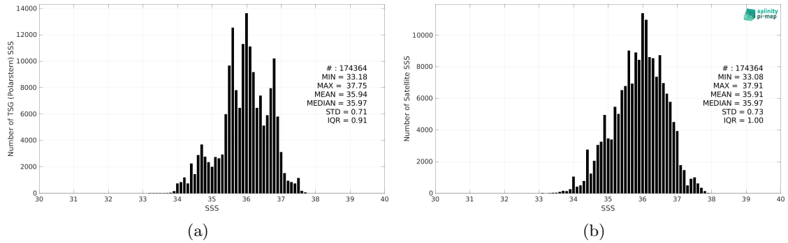
Figure 2: Histograms of SSS from TSG (Polarstern) (a) and SMOS SSS L3 v332 - 9 Days (CATDS-CPDC) (b) considering all match-up pairs per bins of 0.1 over the Mid-Low Latitudes 45N-45S Pi-MEP region and for the full satellite product period.
