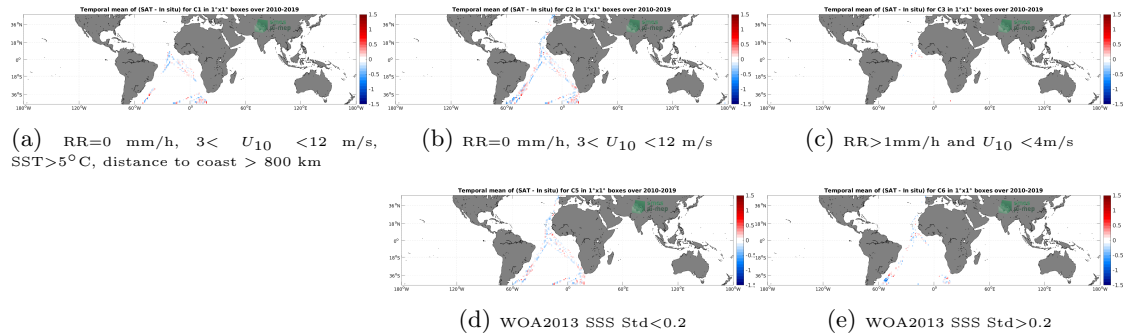
Figure 12: Temporal mean gridded over spatial boxes of size 1^\circ \times 1^\circ of \Delta SSS (SMOS SSS L3 v332 - 9 Days (CATDS-CPDC) - TSG (Polarstern)) for 5 different subdatasets corresponding to:RR=0 mm/h, 3 < U_{10} < 12 m/s, SST > 5^\circ C , distance to coast > 800 km (a), RR=0 mm/h, 3 < U_{10} < 12 m/s (b), RR > 1 mm/h and U_{10} < 4 m/s (c), WOA2013 SSS Std <0.2 (d), WOA2013 SSS Std >0.2 (e).
