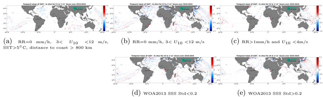
Figure 14: Temporal mean gridded over spatial boxes of size 1^\circ \times 1^\circ of \Delta\text{SSS} (SMOS SSS L3 v332 - 9 Days (CATDS-CPDC) - TSG (LEGOS-DM)) for 5 different subdatasets corresponding to: RR=0 mm/h, 3 < U_{10} < 12 m/s, SST > 5°C, distance to coast > 800 km (a), RR=0 mm/h, 3 < U_{10} < 12 m/s (b), RR > 1mm/h and U_{10} < 4 m/s (c), WOA2013 SSS Std < 0.2 (d), WOA2013 SSS Std > 0.2 (e).
