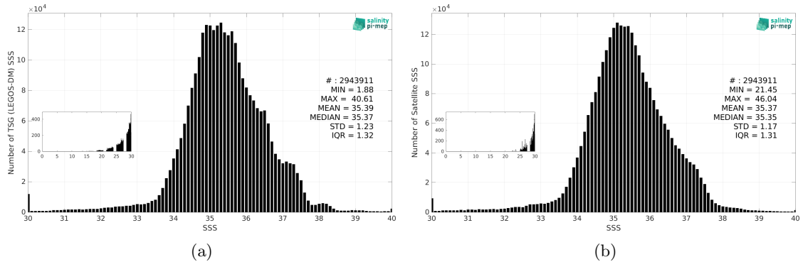
Figure 3: Histograms of SSS from TSG (LEGOS-DM) (a) and SMOS SSS L3 v332 - 9 Days (CATDS-CPDC) (b) considering all match-up pairs per bins of 0.1 over the Mid-Low Latitudes 45N-45S Pi-MEP region and for the full satellite product period.
