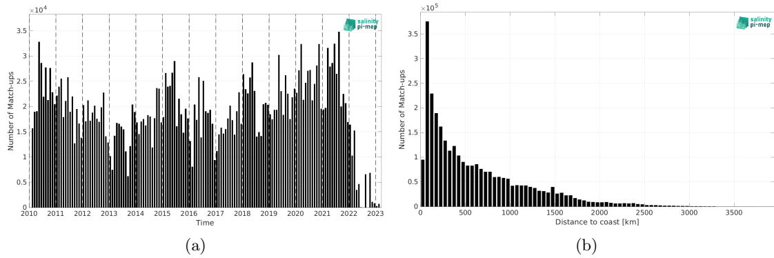
Figure 2: Number of match-ups between TSG (LEGOS-DM) and SMOS SSS L3 v332 - 9 Days (CATDS-CPDC) SSS as a function of time (a) and as function of the distance to coast (b) over the Mid-Low Latitudes 45N-45S Pi-MEP region and for the full satellite product period.
