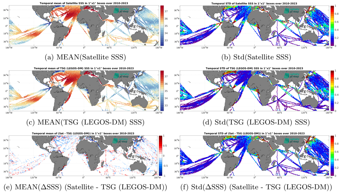
Figure 7: Temporal mean (left) and Std (right) of SSS from SMOS SSS L3 v332 - 9 Days (CATDS-CPDC) (top), TSG (LEGOS-DM) (middle), and of \Delta SSS (Satellite - TSG (LEGOS-DM)). Only match-up pairs are used to generate these maps.
