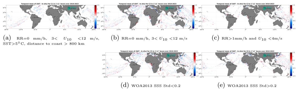
Figure 14: Temporal mean gridded over spatial boxes of size 1^\circ \times 1^\circ of \Delta SSS (SMOS SSS L3 v332 - 9 Days (CATDS-CPDC) - TSG (LEGOS-DM)) for 5 different subdatasets corresponding to:RR=0 mm/h, 3 < U_{10} < 12 m/s, SST >5^\circ\text{C} , distance to coast > 800 km (a), RR=0 mm/h, 3 < U_{10} < 12 m/s (b), RR >1 mm/h and U_{10} < 4 m/s (c), WOA2013 SSS Std <0.2 (d), WOA2013 SSS Std >0.2 (e).
