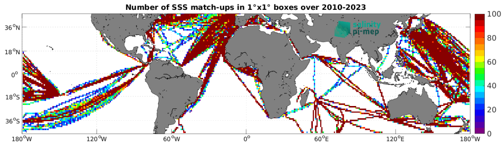
Figure 5: Number of SSS match-ups between TSG (LEGOS-DM) SSS and the SMOS SSS L3 v332 - 9 Days (CATDS-CPDC) SSS product for the Mid-Low Latitudes 45N-45S Pi-MEP region over 1^\circ \times 1^\circ boxes and for the full satellite product period.
