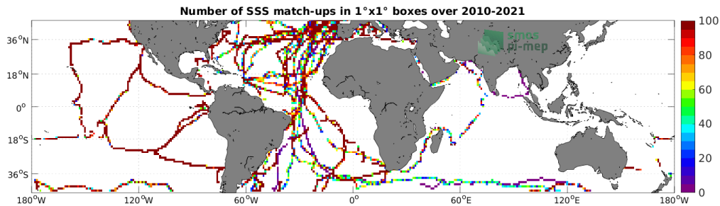
Figure 4: Number of SSS match-ups between TSG (GOSUD-Sailing-ship) SSS and the SMOS SSS L3 v332 - 9 Days (CATDS-CPDC) SSS product for the Mid-Low Latitudes 45N-45S Pi-MEP region over 1^\circ \times 1^\circ boxes and for the full satellite product period.
