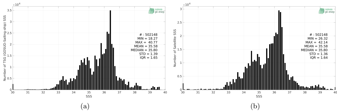
Figure 2: Histograms of SSS from TSG (GOSUD-Sailing-ship) (a) and SMOS SSS L3 v332 - 9 Days (CATDS-CPDC) (b) considering all match-up pairs per bins of 0.1 over the Mid-Low Latitudes 45N-45S Pi-MEP region and for the full satellite product period.
