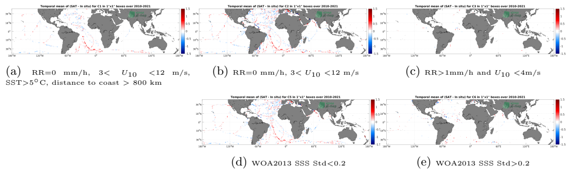
Figure 12: Temporal mean gridded over spatial boxes of size 1^\circ \times 1^\circ of \Delta SSS (SMOS SSS L3 v332 - 9 Days (CATDS-CPDC) - TSG (GOSUD-Sailing-ship)) for 5 different subdatasets corresponding to:RR=0 mm/h, 3 < U_{10} < 12 m/s, SST >5^\circ C, distance to coast > 800 km (a), RR=0 mm/h, 3 < U_{10} < 12 m/s (b), RR >1 mm/h and U_{10} < 4 m/s (c), WOA2013 SSS Std <0.2 (d), WOA2013 SSS Std >0.2 (e).
