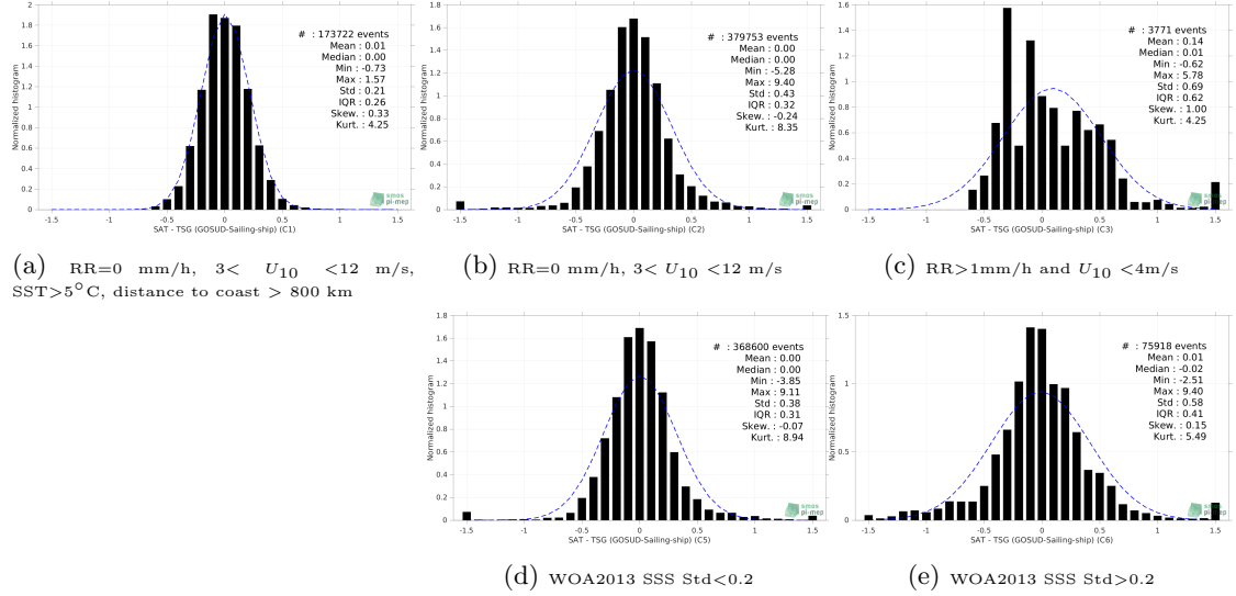
Figure 13: Normalized histogram of \Delta\text{SSS} (SMOS SSS L3 v332 - 9 Days (CATDS-CPDC) - TSG (GOSUD-Sailing-ship)) for 5 different subdatasets corresponding to: RR=0 mm/h, 3 < U_{10} < 12 m/s, SST >5^{\circ}\text{C} , distance to coast > 800 km (a), RR=0 mm/h, 3 < U_{10} < 12 m/s (b), RR >1 mm/h and U_{10} < 4 m/s (c), WOA2013 SSS Std <0.2 (d), WOA2013 SSS Std >0.2 (e).
