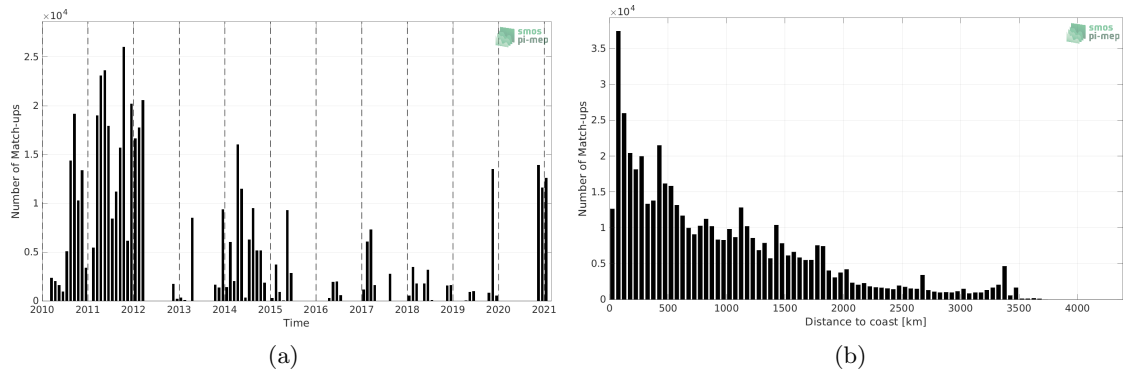
Figure 1: Number of match-ups between TSG (GOSUD-Sailing-ship) and SMOS SSS L3 v332 - 9 Days (CATDS-CPDC) SSS as a function of time (a) and as function of the distance to coast (b) over the Mid-Low Latitudes 45N-45S Pi-MEP region and for the full satellite product period.
