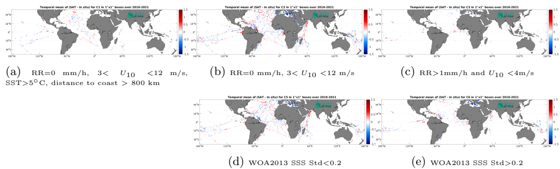
Figure 14: Temporal mean gridded over spatial boxes of size 1^\circ \times 1^\circ of \Delta SSS (SMOS SSS L3 v332 - 9 Days (CATDS-CPDC) - TSG (GOSUD-Research-vessel)) for 5 different subdatasets corresponding to: RR=0 mm/h, 3 < U_{10} < 12 m/s, SST > 5°C, distance to coast > 800 km (a), RR=0 mm/h, 3 < U_{10} < 12 m/s (b), RR > 1mm/h and U_{10} < 4 m/s (c), WOA2013 SSS Std < 0.2 (d), WOA2013 SSS Std > 0.2 (e).
