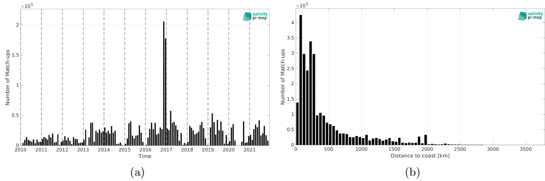
Figure 2: Number of match-ups between TSG (GOSUD-Research-vessel) and SMOS SSS L3 v332 - 9 Days (CATDS-CPDC) SSS as a function of time (a) and as function of the distance to coast (b) over the Mid-Low Latitudes 45N-45S Pi-MEP region and for the full satellite product period.
