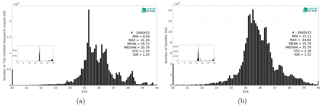
Figure 3: Histograms of SSS from TSG (GOSUD-Research-vessel) (a) and SMOS SSS L3 v332 - 9 Days (CATDS-CPDC) (b) considering all match-up pairs per bins of 0.1 over the Mid-Low Latitudes 45N-45S Pi-MEP region and for the full satellite product period.
