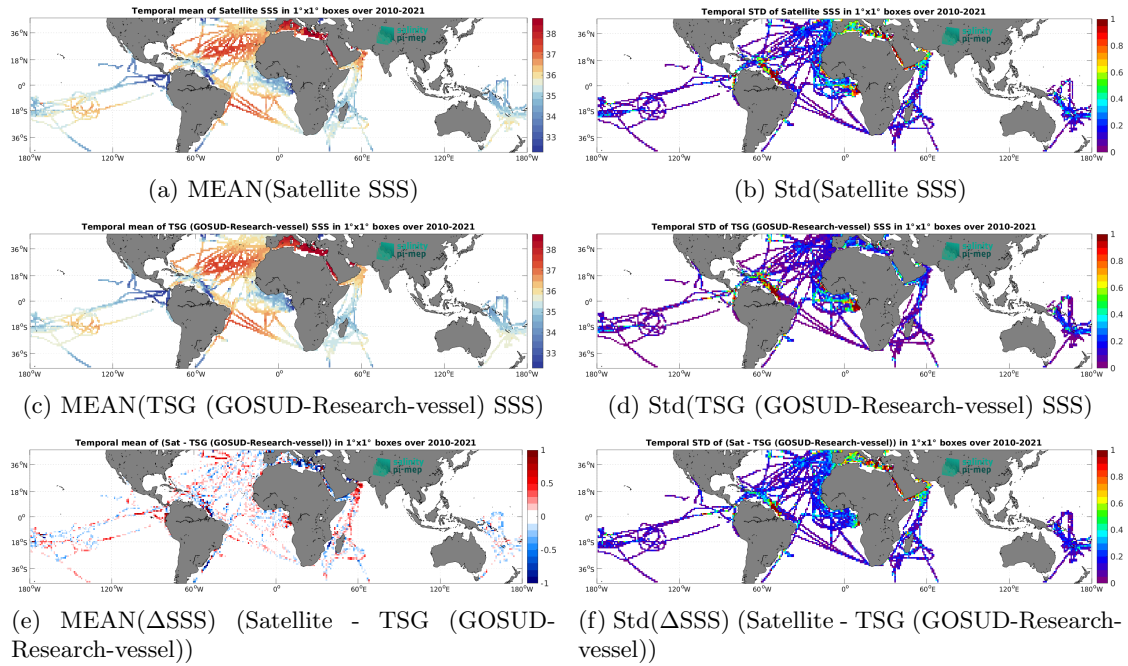
Figure 7: Temporal mean (left) and Std (right) of SSS from SMOS SSS L3 v332 - 9 Days (CATDS-CPDC) (top), TSG (GOSUD-Research-vessel) (middle), and of \Delta SSS (Satellite - TSG (GOSUD-Research-vessel)). Only match-up pairs are used to generate these maps.
