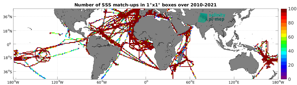
Figure 5: Number of SSS match-ups between TSG (GOSUD-Research-vessel) SSS and the SMOS SSS L3 v332 - 9 Days (CATDS-CPDC) SSS product for the Mid-Low Latitudes 45N-45S Pi-MEP region over 1^\circ \times 1^\circ boxes and for the full satellite product period.
