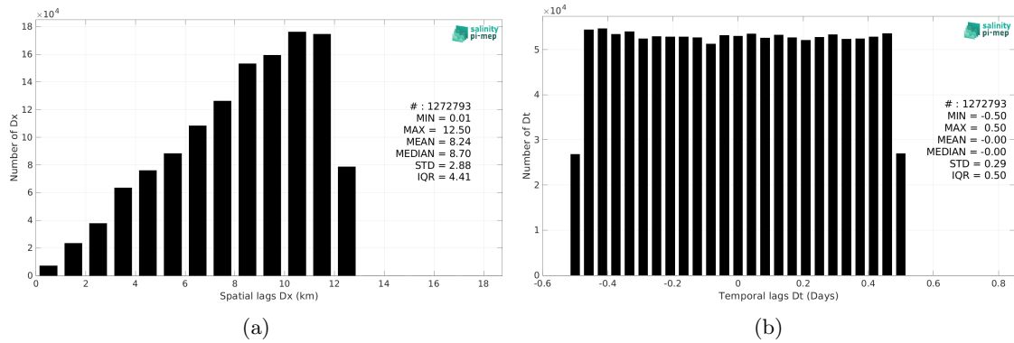
Figure 5: Histograms of the spatial (a) and temporal (b) lags between the location/time of the TSG (CSIC-UTM) measurement and the date of the corresponding SMOS SSS L3 v332 - 9 Days (CATDS-CPDC) SSS pixel.
