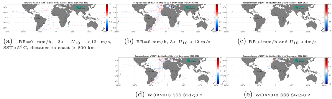
Figure 12: Temporal mean gridded over spatial boxes of size 1^\circ \times 1^\circ of \Delta SSS (SMOS SSS L3 v332 - 9 Days (CATDS-CPDC) - TSG (CSIC-UTM)) for 5 different subdatasets corresponding to:RR=0 mm/h, 3 < U_{10} < 12 m/s, SST >5^\circ\text{C} , distance to coast > 800 km (a), RR=0 mm/h, 3 < U_{10} < 12 m/s (b), RR >1 mm/h and U_{10} < 4 m/s (c), WOA2013 SSS Std <0.2 (d), WOA2013 SSS Std >0.2 (e).
