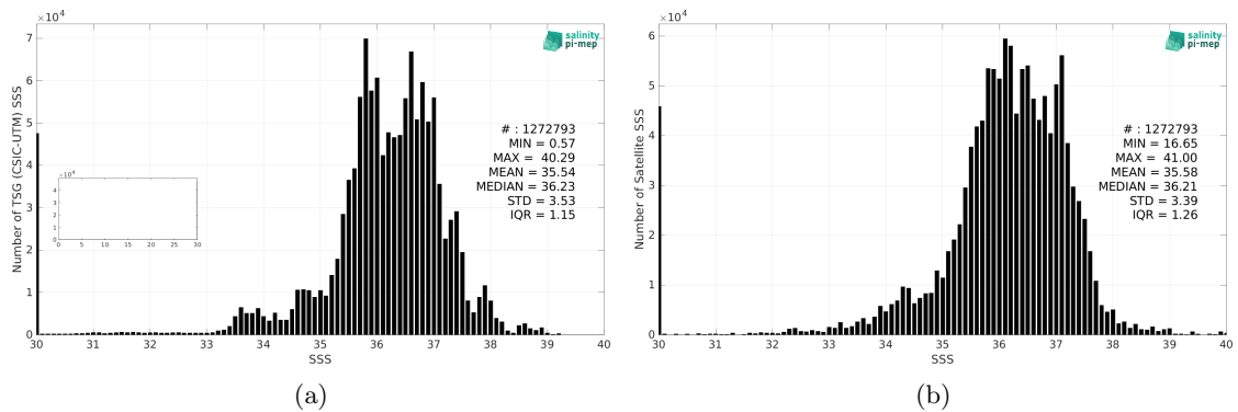
Figure 2: Histograms of SSS from TSG (CSIC-UTM) (a) and SMOS SSS L3 v332 - 9 Days (CATDS-CPDC) (b) considering all match-up pairs per bins of 0.1 over the Mid-Low Latitudes 45N-45S Pi-MEP region and for the full satellite product period.
