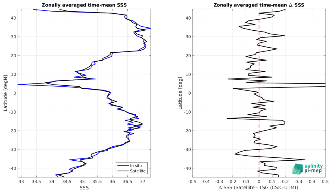
Figure 8: Left panel: Zonal mean SSS from SMOS SSS L3 v332 - 9 Days (CATDS-CPDC) satellite product (black) and from TSG (CSIC-UTM) (blue). Right panel: Zonal mean of \Delta SSS (Satellite - TSG (CSIC-UTM)) for all the collected Pi-MEP match-up pairs estimated over the full satellite product period.
