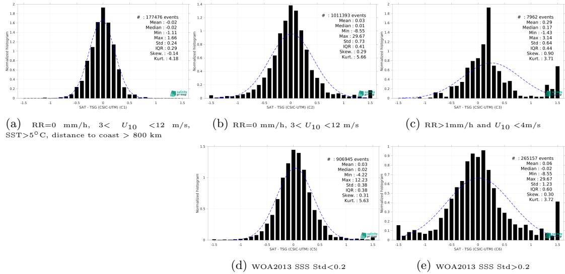
Figure 13: Normalized histogram of \Delta SSS (SMOS SSS L3 v332 - 9 Days (CATDS-CPDC) - TSG (CSIC-UTM)) for 5 different subdatasets corresponding to: RR=0 mm/h, 3 < U_{10} < 12 m/s, SST>5°C, distance to coast > 800 km (a), RR=0 mm/h, 3 < U_{10} < 12 m/s (b), RR>1mm/h and U_{10} < 4 m/s (c), WOA2013 SSS Std<0.2 (d), WOA2013 SSS Std>0.2 (e).
