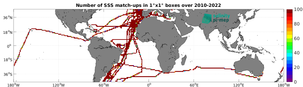
Figure 4: Number of SSS match-ups between TSG (CSIC-UTM) SSS and the SMOS SSS L3 v332 - 9 Days (CATDS-CPDC) SSS product for the Mid-Low Latitudes 45N-45S Pi-MEP region over 1^\circ \times 1^\circ boxes and for the full satellite product period.
