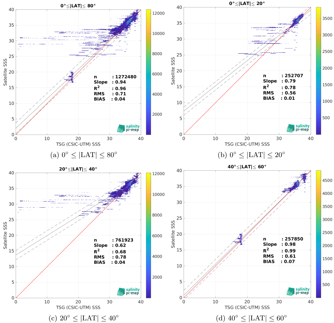
Figure 9: Contour maps of the concentration of SMOS SSS L3 v332 - 9 Days (CATDS-CPDC) SSS (y-axis) versus TSG (CSIC-UTM) SSS (x-axis) at match-up pairs for different latitude bands. For each plot, the red line shows x=y . The black thin and dashed lines indicate a linear fit through the data cloud and the \pm 95\% confidence levels, respectively. The number match-up pairs n , the slope and R^2 coefficient of the linear fit, the root mean square (RMS) and the mean bias between satellite and in situ data are indicated for each latitude band in each plots.
