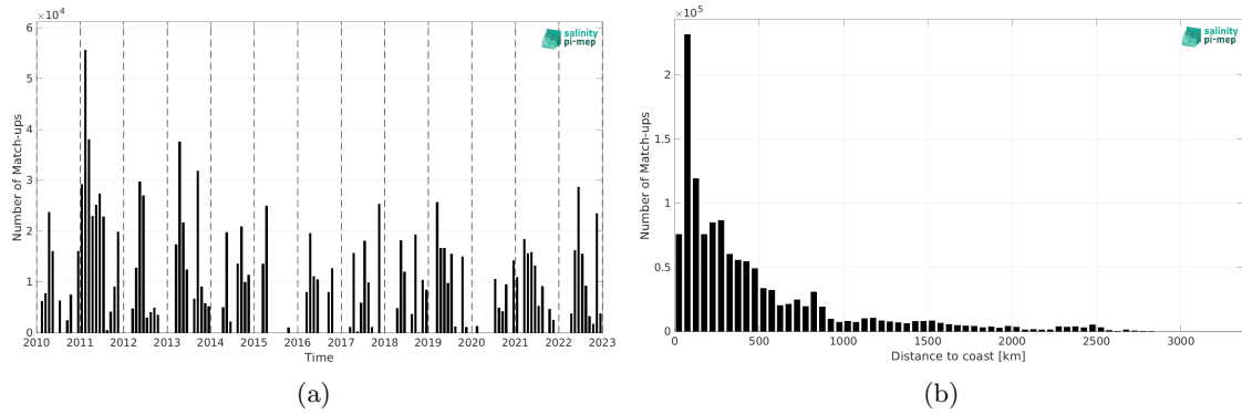
Figure 1: Number of match-ups between TSG (CSIC-UTM) and SMOS SSS L3 v332 - 9 Days (CATDS-CPDC) SSS as a function of time (a) and as function of the distance to coast (b) over the Mid-Low Latitudes 45N-45S Pi-MEP region and for the full satellite product period.
