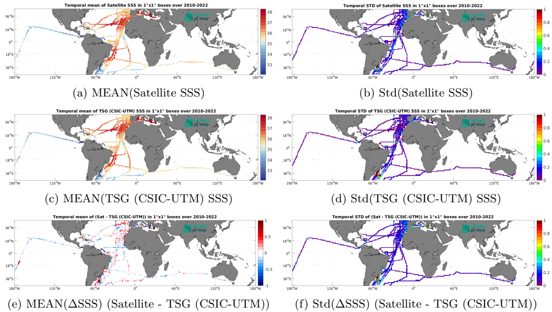
Figure 6: Temporal mean (left) and Std (right) of SSS from SMOS SSS L3 v332 - 9 Days (CATDS-CPDC) (top), TSG (CSIC-UTM) (middle), and of \Delta SSS (Satellite - TSG (CSIC-UTM)). Only match-up pairs are used to generate these maps.
