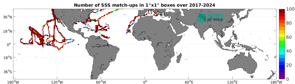
Figure 5: Number of SSS match-ups between Saildrone SSS and the SMOS SSS L3 v332 - 9 Days (CATDS-CPDC) SSS product for the Mid-Low Latitudes 45N-45S Pi-MEP region over 1^\circ \times 1^\circ boxes and for the full satellite product period.
