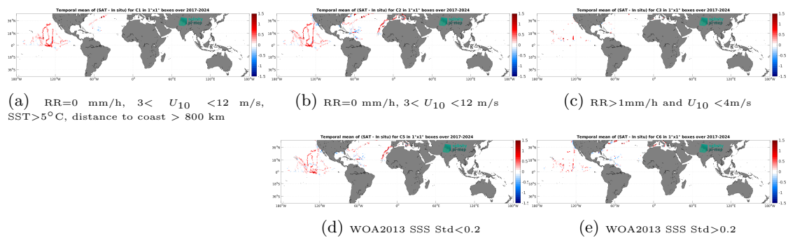
Figure 14: Temporal mean gridded over spatial boxes of size 1^\circ \times 1^\circ of \Delta SSS (SMOS SSS L3 v332 - 9 Days (CATDS-CPDC) - Sairdrone) for 5 different subdatasets corresponding to: RR=0 mm/h, 3 < U_{10} < 12 m/s, SST > 5^\circ\text{C} , distance to coast > 800 km (a), RR=0 mm/h, 3 < U_{10} < 12 m/s (b), RR > 1 mm/h and U_{10} < 4 m/s (c), WOA2013 SSS Std < 0.2 (d), WOA2013 SSS Std > 0.2 (e).
