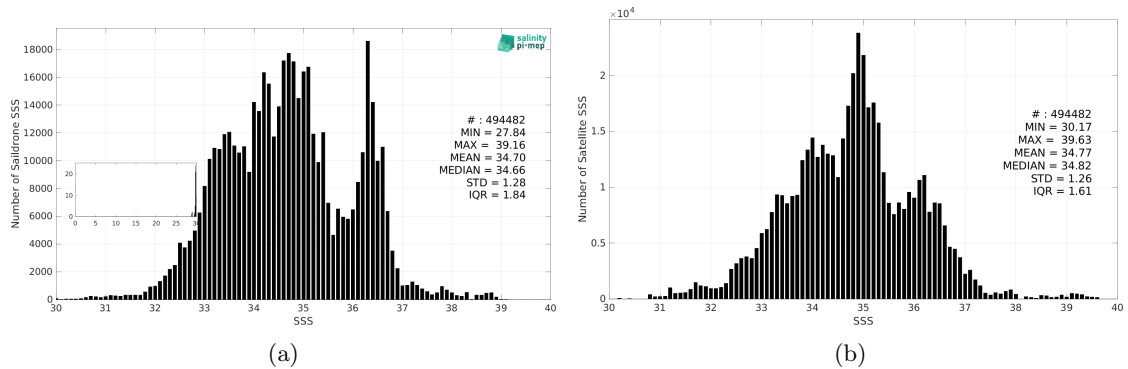
Figure 3: Histograms of SSS from Saildrone (a) and SMOS SSS L3 v332 - 9 Days (CATDS-CPDC) (b) considering all match-up pairs per bins of 0.1 over the Mid-Low Latitudes 45N-45S Pi-MEP region and for the full satellite product period.
