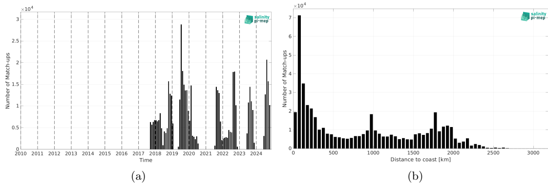
Figure 2: Number of match-ups between Saildrone and SMOS SSS L3 v332 - 9 Days (CATDS-CPDC) SSS as a function of time (a) and as function of the distance to coast (b) over the Mid-Low Latitudes 45N-45S Pi-MEP region and for the full satellite product period.
