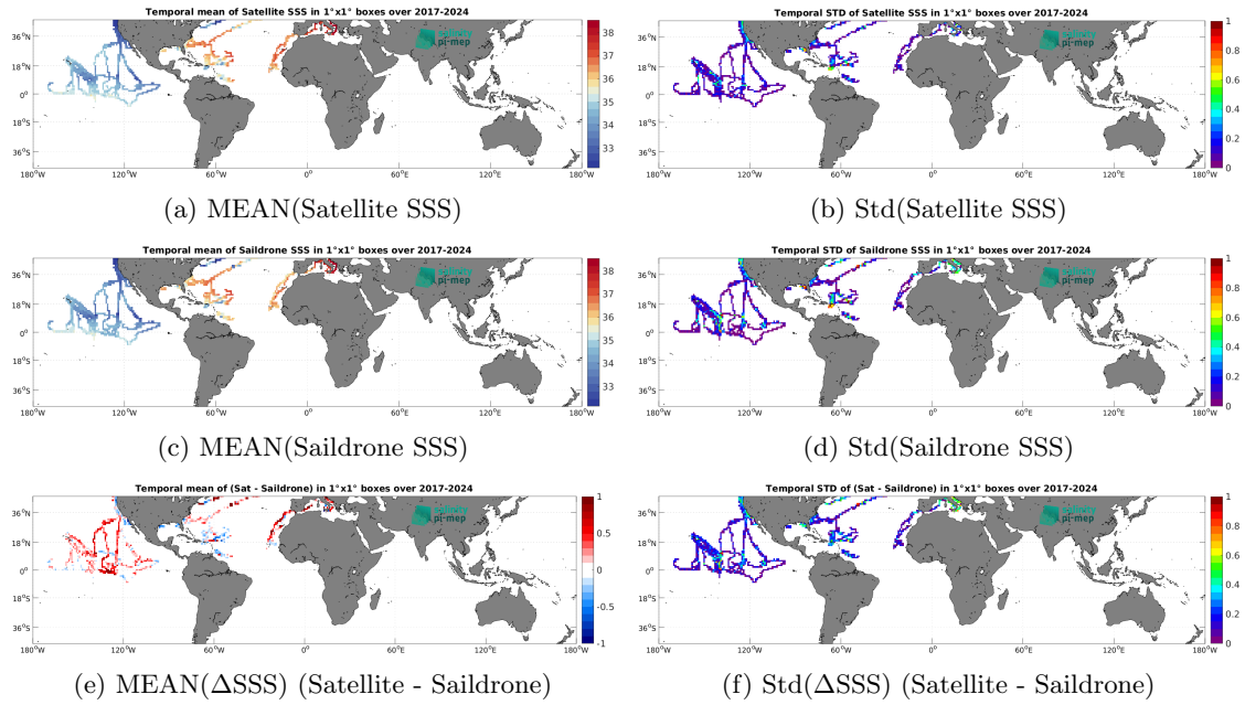
Figure 7: Temporal mean (left) and Std (right) of SSS from SMOS SSS L3 v332 - 9 Days (CATDS-CPDC) (top), Saildrone (middle), and of \Delta SSS (Satellite - Saildrone). Only match-up pairs are used to generate these maps.
