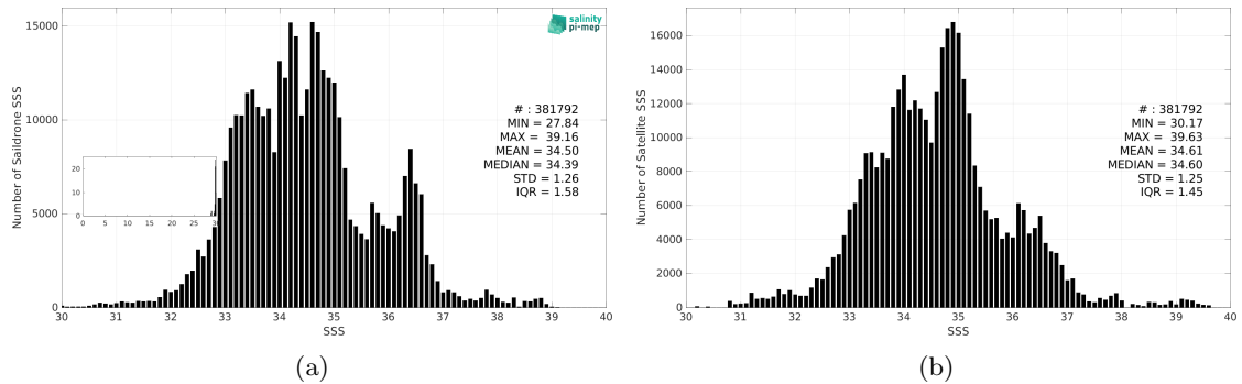
Figure 3: Histograms of SSS from Saildrone (a) and SMOS SSS L3 v332 - 9 Days (CATDS-CPDC) (b) considering all match-up pairs per bins of 0.1 over the Mid-Low Latitudes 45N-45S Pi-MEP region and for the full satellite product period.
