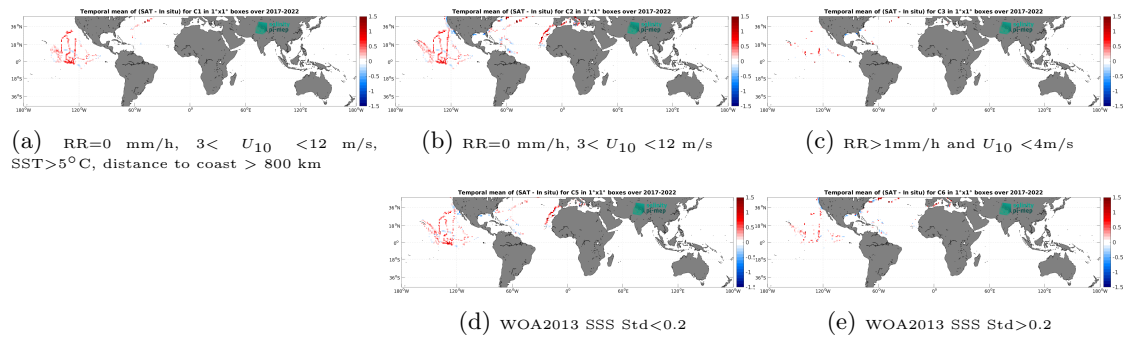
Figure 12: Temporal mean gridded over spatial boxes of size 1^\circ \times 1^\circ of \Delta\text{SSS} (SMOS SSS L3 v332 - 9 Days (CATDS-CPDC) - Sairdrone) for 5 different subdatasets corresponding to: RR=0 mm/h, 3 < U_{10} < 12 m/s, SST > 5^\circ\text{C} , distance to coast > 800 km (a), RR=0 mm/h, 3 < U_{10} < 12 m/s (b), RR > 1 mm/h and U_{10} < 4 m/s (c), WOA2013 SSS Std < 0.2 (d), WOA2013 SSS Std > 0.2 (e).
