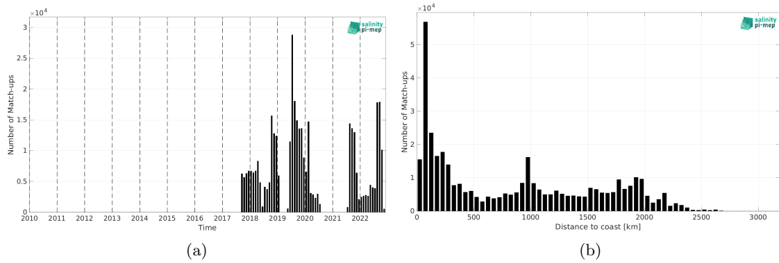
Figure 1: Number of match-ups between Sailldrone and SMOS SSS L3 v332 - 9 Days (CATDS-CPDC) SSS as a function of time (a) and as function of the distance to coast (b) over the Mid-Low Latitudes 45N-45S Pi-MEP region and for the full satellite product period.
