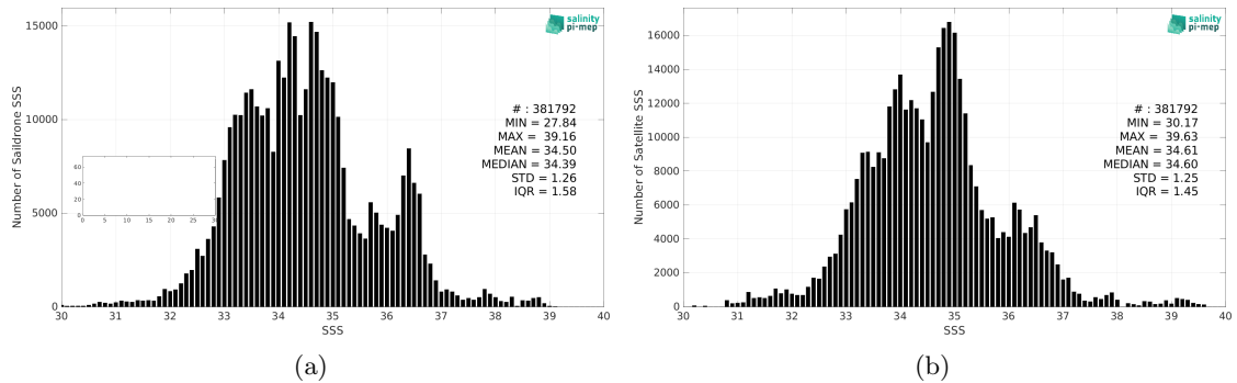
Figure 2: Histograms of SSS from Sailldrone (a) and SMOS SSS L3 v332 - 9 Days (CATDS-CPDC) (b) considering all match-up pairs per bins of 0.1 over the Mid-Low Latitudes 45N-45S Pi-MEP region and for the full satellite product period.
