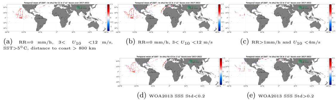
Figure 12: Temporal mean gridded over spatial boxes of size 1^\circ \times 1^\circ of \Delta SSS (SMOS SSS L3 v332 - 9 Days (CATDS-CPDC) - Sairdrone) for 5 different subdatasets corresponding to:RR=0 mm/h, 3 < U_{10} < 12 m/s, SST >5^\circ C, distance to coast > 800 km (a), RR=0 mm/h, 3 < U_{10} < 12 m/s (b), RR >1 mm/h and U_{10} < 4 m/s (c), WOA2013 SSS Std <0.2 (d), WOA2013 SSS Std >0.2 (e).
