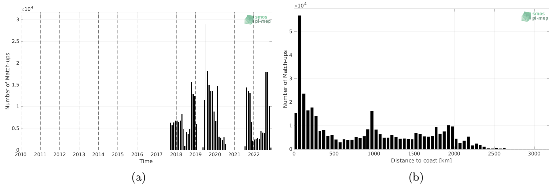
Figure 1: Number of match-ups between Saïdrone and SMOS SSS L3 v332 - 9 Days (CATDS-CPDC) SSS as a function of time (a) and as function of the distance to coast (b) over the Mid-Low Latitudes 45N-45S Pi-MEP region and for the full satellite product period.
