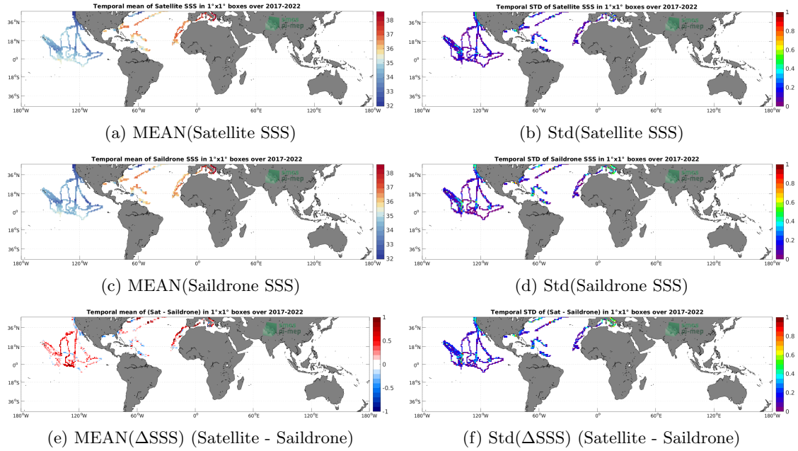
Figure 6: Temporal mean (left) and Std (right) of SSS from SMOS SSS L3 v332 - 9 Days (CATDS-CPDC) (top), Saildrone (middle), and of \Delta SSS (Satellite - Saildrone). Only match-up pairs are used to generate these maps.
