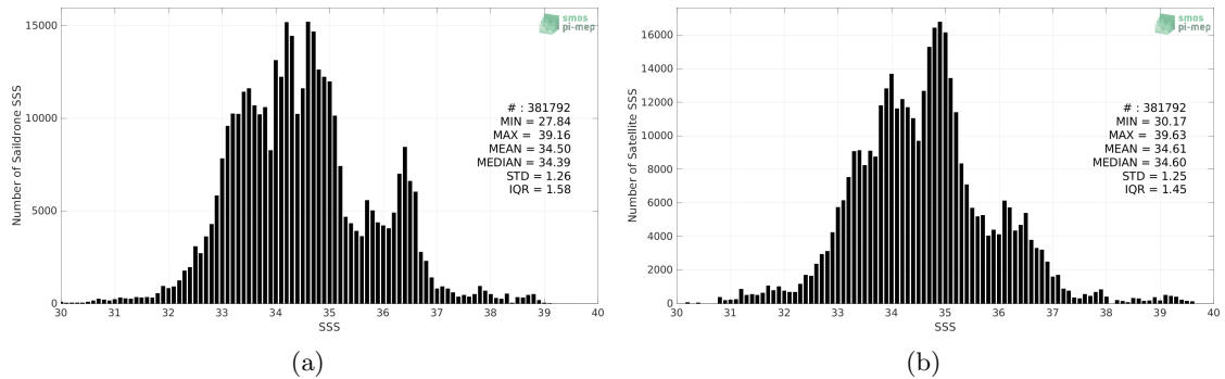
Figure 2: Histograms of SSS from Saïdrone (a) and SMOS SSS L3 v332 - 9 Days (CATDS-CPDC) (b) considering all match-up pairs per bins of 0.1 over the Mid-Low Latitudes 45N-45S Pi-MEP region and for the full satellite product period.
