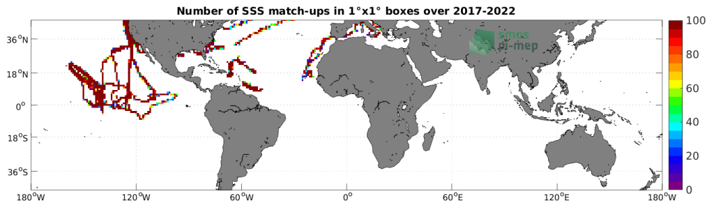
Figure 4: Number of SSS match-ups between Saildrone SSS and the SMOS SSS L3 v332 - 9 Days (CATDS-CPDC) SSS product for the Mid-Low Latitudes 45N-45S Pi-MEP region over 1^\circ \times 1^\circ boxes and for the full satellite product period.
