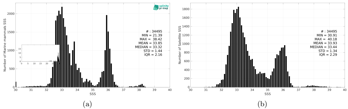
Figure 3: Histograms of SSS from Marine mammals (a) and SMOS SSS L3 v332 - 9 Days (CATDS-CPDC) (b) considering all match-up pairs per bins of 0.1 over the Mid-Low Latitudes 45N-45S Pi-MEP region and for the full satellite product period.
