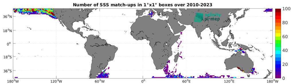
Figure 5: Number of SSS match-ups between Marine mammals SSS and the SMOS SSS L3 v332 - 9 Days (CATDS-CPDC) SSS product for the Mid-Low Latitudes 45N-45S Pi-MEP region over 1^\circ \times 1^\circ boxes and for the full satellite product period.
