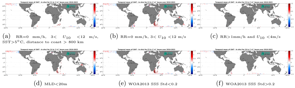
Figure 14: Temporal mean gridded over spatial boxes of size 1^\circ \times 1^\circ of \Delta SSS (SMOS SSS L3 v332 - 9 Days (CATDS-CPDC) - Marine mammals) for 6 different subdatasets corresponding to:RR=0 mm/h, 3 < U_{10} < 12 m/s, SST>5°C, distance to coast > 800 km (a), RR=0 mm/h, 3 < U_{10} < 12 m/s (b), RR>1mm/h and U_{10} < 4 m/s (c),MLD<20m (d),WOA2013 SSS Std<0.2 (e),WOA2013 SSS Std>0.2 (f).
