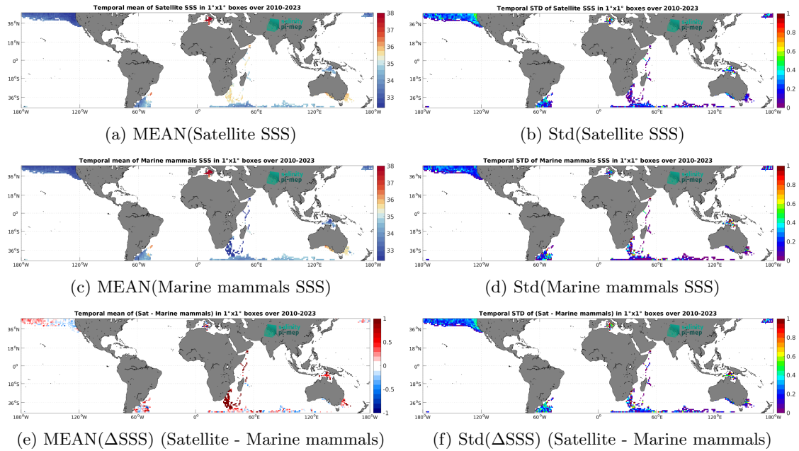
Figure 7: Temporal mean (left) and Std (right) of SSS from SMOS SSS L3 v332 - 9 Days (CATDS-CPDC) (top), Marine mammals (middle), and of \Delta SSS (Satellite - Marine mammals). Only match-up pairs are used to generate these maps.
