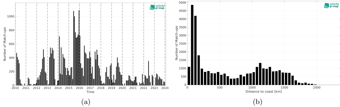
Figure 2: Number of match-ups between Marine mammals and SMOS SSS L3 v332 - 9 Days (CATDS-CPDC) SSS as a function of time (a) and as function of the distance to coast (b) over the Mid-Low Latitudes 45N-45S Pi-MEP region and for the full satellite product period.
