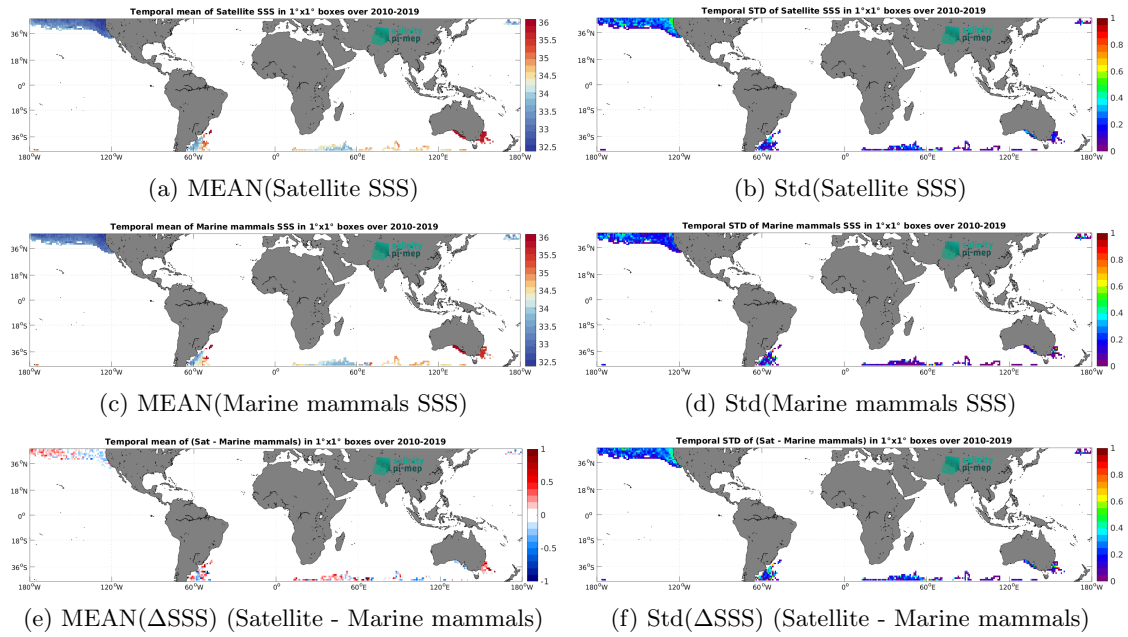
Figure 6: Temporal mean (left) and Std (right) of SSS from SMOS SSS L3 v332 - 9 Days (CATDS-CPDC) (top), Marine mammals (middle), and of \Delta SSS (Satellite - Marine mammals). Only match-up pairs are used to generate these maps.
