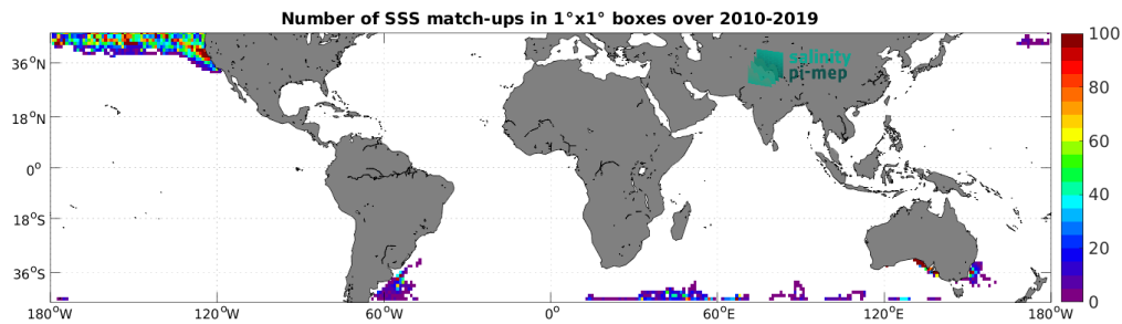
Figure 4: Number of SSS match-ups between Marine mammals SSS and the SMOS SSS L3 v332 - 9 Days (CATDS-CPDC) SSS product for the Mid-Low Latitudes 45N-45S Pi-MEP region over 1^\circ \times 1^\circ boxes and for the full satellite product period.
