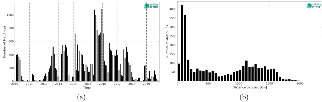
Figure 1: Number of match-ups between Marine mammals and SMOS SSS L3 v332 - 9 Days (CATDS-CPDC) SSS as a function of time (a) and as function of the distance to coast (b) over the Mid-Low Latitudes 45N-45S Pi-MEP region and for the full satellite product period.
