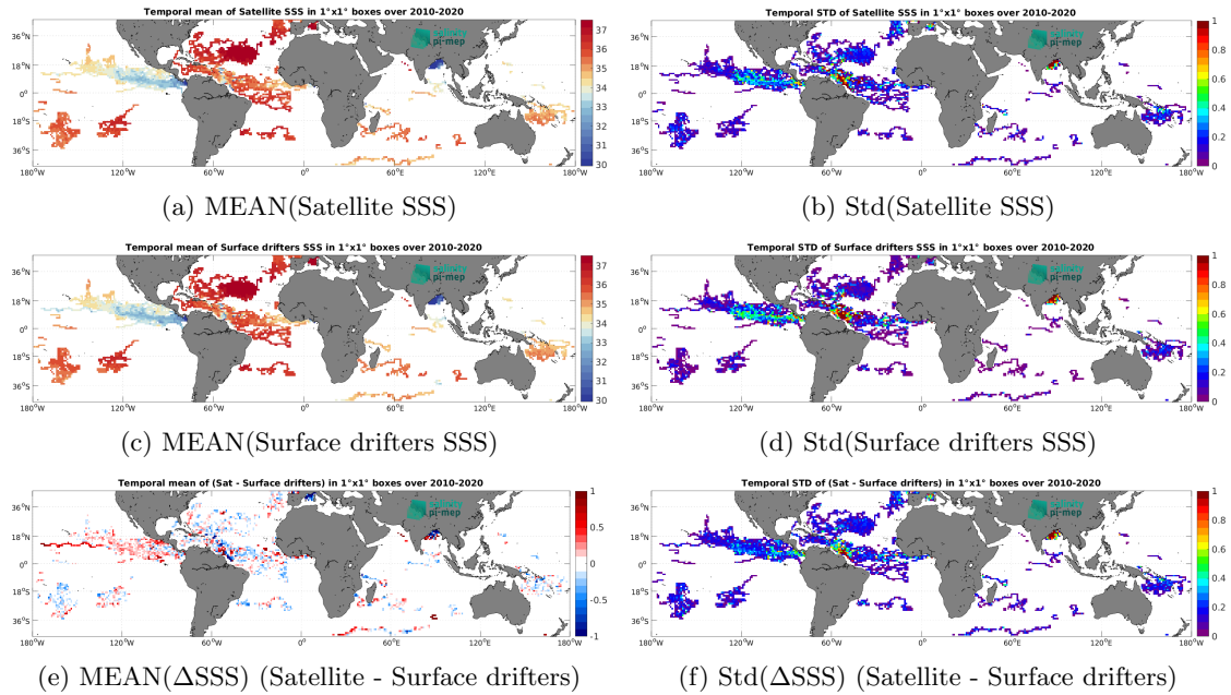
Figure 6: Temporal mean (left) and Std (right) of SSS from SMOS SSS L3 v332 - 9 Days (CATDS-CPDC) (top), Surface drifters (middle), and of \Delta SSS (Satellite - Surface drifters). Only match-up pairs are used to generate these maps.
