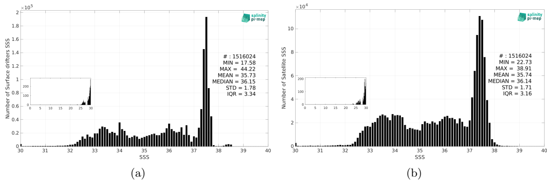
Figure 3: Histograms of SSS from Surface drifters (a) and SMOS SSS L3 v332 - 9 Days (CATDS-CPDC) (b) considering all match-up pairs per bins of 0.1 over the Mid-Low Latitudes 45N-45S Pi-MEP region and for the full satellite product period.
