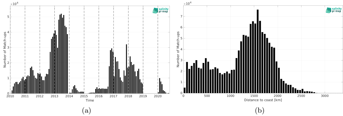
Figure 2: Number of match-ups between Surface drifters and SMOS SSS L3 v332 - 9 Days (CATDS-CPDC) SSS as a function of time (a) and as function of the distance to coast (b) over the Mid-Low Latitudes 45N-45S Pi-MEP region and for the full satellite product period.
