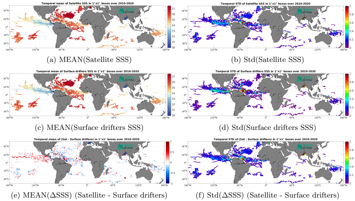
Figure 5: Temporal mean (left) and Std (right) of SSS from SMOS SSS L3 v332 - 9 Days (CATDS-CPDC) (top), Surface drifters (middle), and of \Delta SSS (Satellite - Surface drifters). Only match-up pairs are used to generate these maps.
