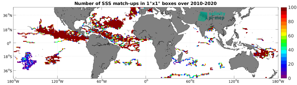
Figure 3: Number of SSS match-ups between Surface drifters SSS and the SMOS SSS L3 v332 - 9 Days (CATDS-CPDC) SSS product for the Mid-Low Latitudes 45N-45S Pi-MEP region over 1^\circ \times 1^\circ boxes and for the full satellite product period.
