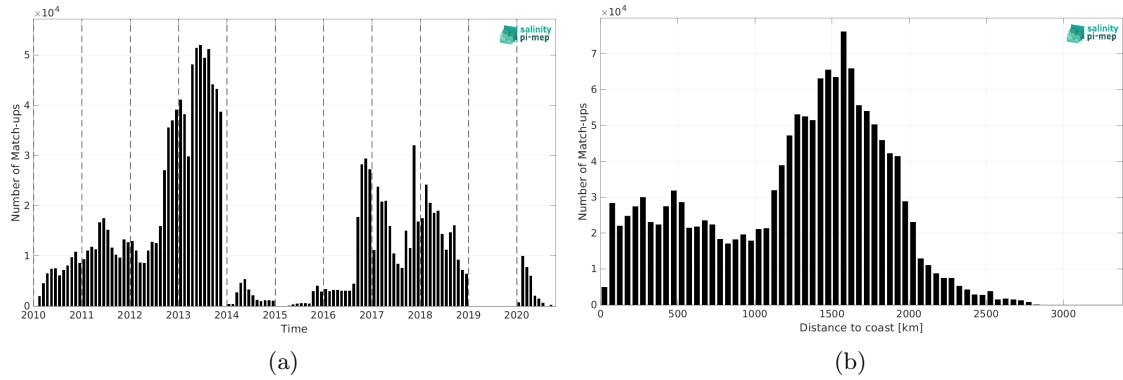
Figure 1: Number of match-ups between Surface drifters and SMOS SSS L3 v332 - 9 Days (CATDS-CPDC) SSS as a function of time (a) and as function of the distance to coast (b) over the Mid-Low Latitudes 45N-45S Pi-MEP region and for the full satellite product period.
