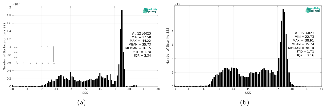
Figure 2: Histograms of SSS from Surface drifters (a) and SMOS SSS L3 v332 - 9 Days (CATDS-CPDC) (b) considering all match-up pairs per bins of 0.1 over the Mid-Low Latitudes 45N-45S Pi-MEP region and for the full satellite product period.
