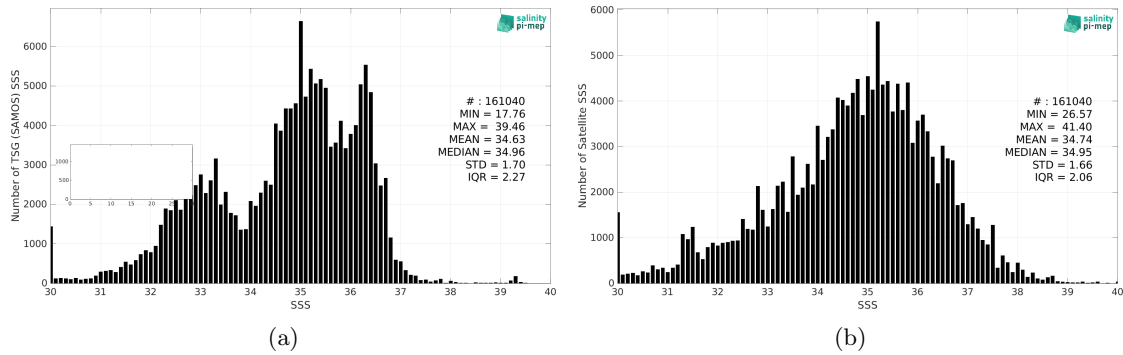
Figure 2: Histograms of SSS from TSG (SAMOS) (a) and SMOS SSS L2Q v331 - 0.25 Deg (CATDS-CPDC) (b) considering all match-up pairs per bins of 0.1 over the Mid-Low Latitudes 45N-45S Pi-MEP region and for the full satellite product period.
