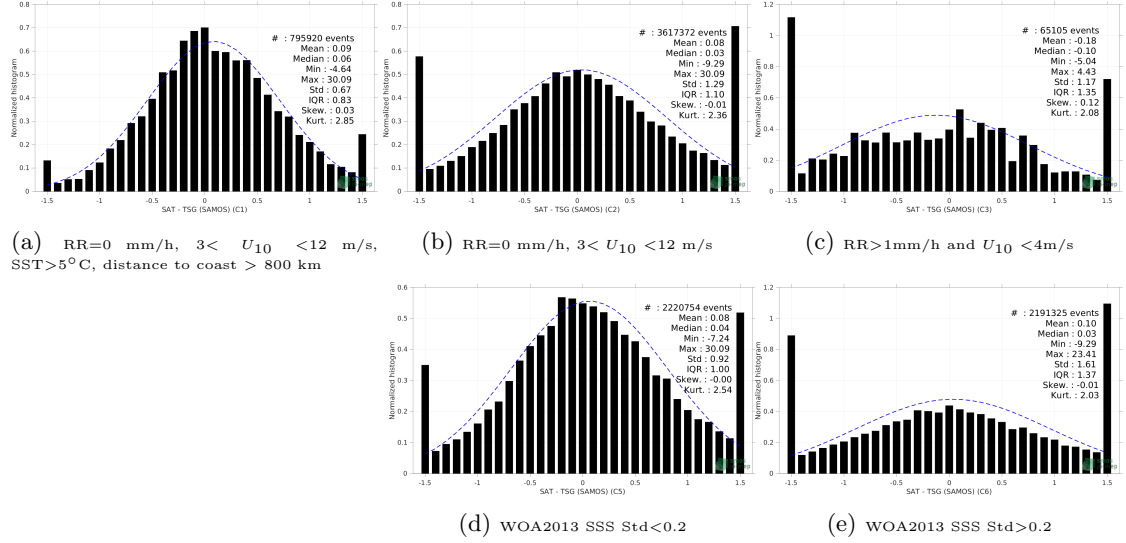
Figure 13: Normalized histogram of \Delta SSS (SMOS SSS L2Q v331 - 0.25 Deg (CATDS-CPDC) - TSG (SAMOS)) for 5 different subdatasets corresponding to: RR=0 mm/h, 3 < U_{10} < 12 m/s, SST>5°C, distance to coast > 800 km (a), RR=0 mm/h, 3 < U_{10} < 12 m/s (b), RR>1mm/h and U_{10} < 4 m/s (c), WOA2013 SSS Std<0.2 (d), WOA2013 SSS Std>0.2 (e).
