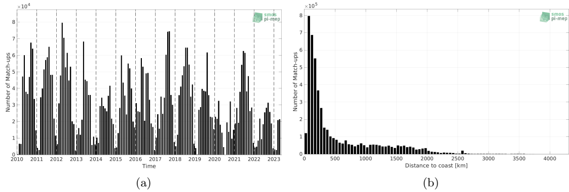
Figure 1: Number of match-ups between TSG (SAMOS) and SMOS SSS L2Q v331 - 0.25 Deg (CATDS-CPDC) SSS as a function of time (a) and as function of the distance to coast (b) over the Mid-Low Latitudes 45N-45S Pi-MEP region and for the full satellite product period.
