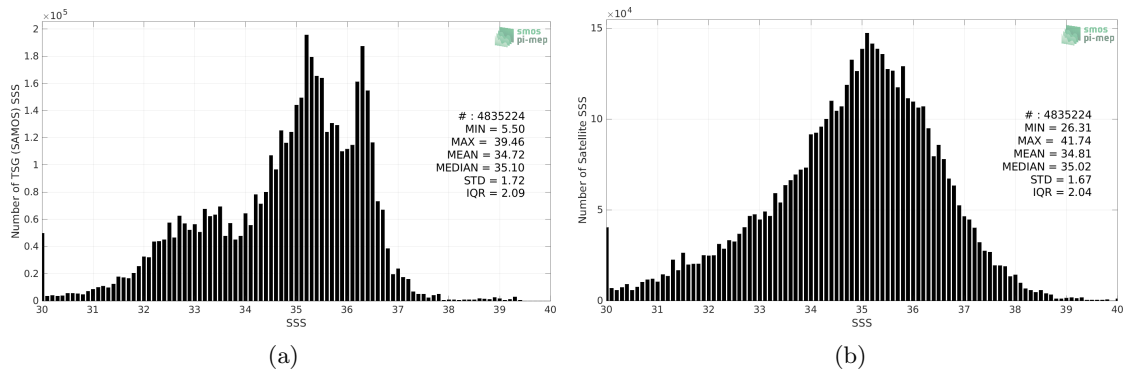
Figure 2: Histograms of SSS from TSG (SAMOS) (a) and SMOS SSS L2Q v331 - 0.25 Deg (CATDS-CPDC) (b) considering all match-up pairs per bins of 0.1 over the Mid-Low Latitudes 45N-45S Pi-MEP region and for the full satellite product period.
