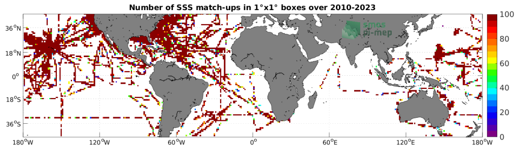
Figure 4: Number of SSS match-ups between TSG (SAMOS) SSS and the SMOS SSS L2Q v331 - 0.25 Deg (CATDS-CPDC) SSS product for the Mid-Low Latitudes 45N-45S Pi-MEP region over 1^\circ \times 1^\circ boxes and for the full satellite product period.
