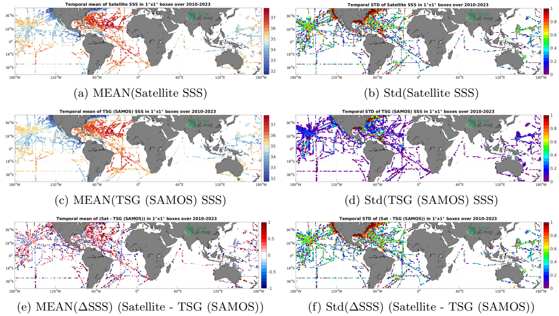
Figure 6: Temporal mean (left) and Std (right) of SSS from SMOS SSS L2Q v331 - 0.25 Deg (CATDS-CPDC) (top), TSG (SAMOS) (middle), and of \Delta SSS (Satellite - TSG (SAMOS)). Only match-up pairs are used to generate these maps.
