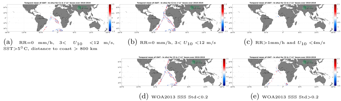
Figure 12: Temporal mean gridded over spatial boxes of size 1^\circ \times 1^\circ of \Delta SSS (SMOS SSS L2Q v331 - 0.25 Deg (CATDS-CPDC) - TSG (Polarstern)) for 5 different subdatasets corresponding to:RR=0 mm/h, 3 < U_{10} < 12 m/s, SST >5^\circ C, distance to coast > 800 km (a), RR=0 mm/h, 3 < U_{10} < 12 m/s (b), RR >1 mm/h and U_{10} < 4 m/s (c), WOA2013 SSS Std <0.2 (d), WOA2013 SSS Std >0.2 (e).
