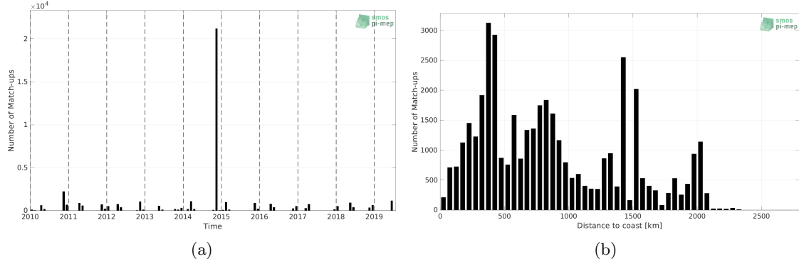
Figure 1: Number of match-ups between TSG (Polarstern) and SMOS SSS L2Q v331 - 0.25 Deg (CATDS-CPDC) SSS as a function of time (a) and as function of the distance to coast (b) over the Mid-Low Latitudes 45N-45S Pi-MEP region and for the full satellite product period.
