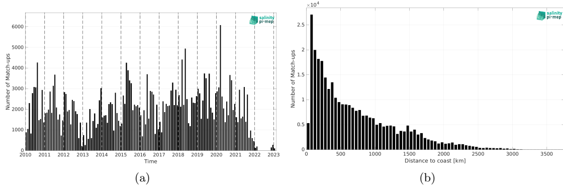
Figure 1: Number of match-ups between TSG (LEGOS-DM) and SMOS SSS L2Q v331 - 0.25 Deg (CATDS-CPDC) SSS as a function of time (a) and as function of the distance to coast (b) over the Mid-Low Latitudes 45N-45S Pi-MEP region and for the full satellite product period.
