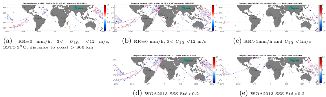
Figure 12: Temporal mean gridded over spatial boxes of size 1^\circ \times 1^\circ of \Delta\text{SSS} (SMOS SSS L2Q v331 - 0.25 Deg (CATDS-CPDC) - TSG (LEGOS-DM)) for 5 different subdatasets corresponding to:RR=0 mm/h, 3 < U_{10} < 12 m/s, SST >5^\circ\text{C} , distance to coast > 800 km (a), RR=0 mm/h, 3 < U_{10} < 12 m/s (b), RR >1 mm/h and U_{10} < 4 m/s (c), WOA2013 SSS Std <0.2 (d), WOA2013 SSS Std >0.2 (e).
