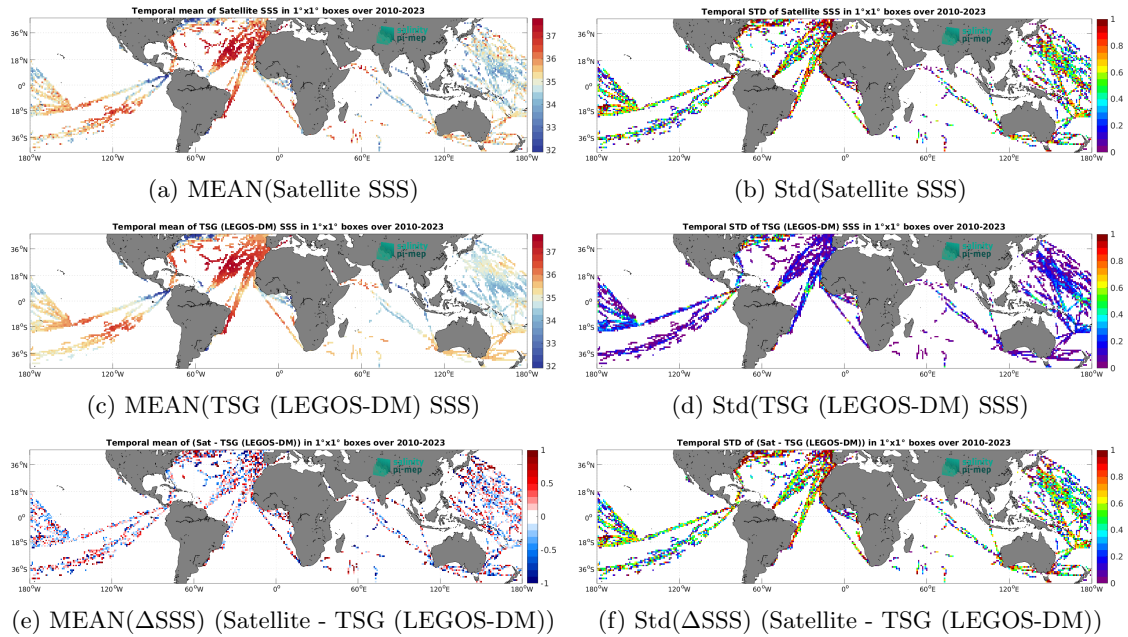
Figure 6: Temporal mean (left) and Std (right) of SSS from SMOS SSS L2Q v331 - 0.25 Deg (CATDS-CPDC) (top), TSG (LEGOS-DM) (middle), and of \Delta SSS (Satellite - TSG (LEGOS-DM)). Only match-up pairs are used to generate these maps.
