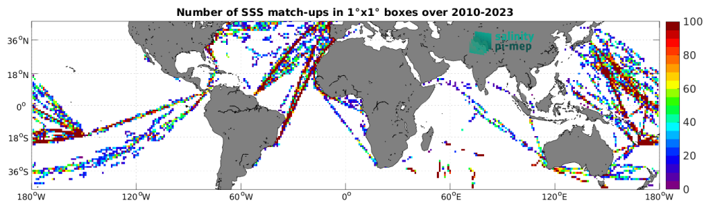
Figure 4: Number of SSS match-ups between TSG (LEGOS-DM) SSS and the SMOS SSS L2Q v331 - 0.25 Deg (CATDS-CPDC) SSS product for the Mid-Low Latitudes 45N-45S Pi-MEP region over 1^\circ \times 1^\circ boxes and for the full satellite product period.
