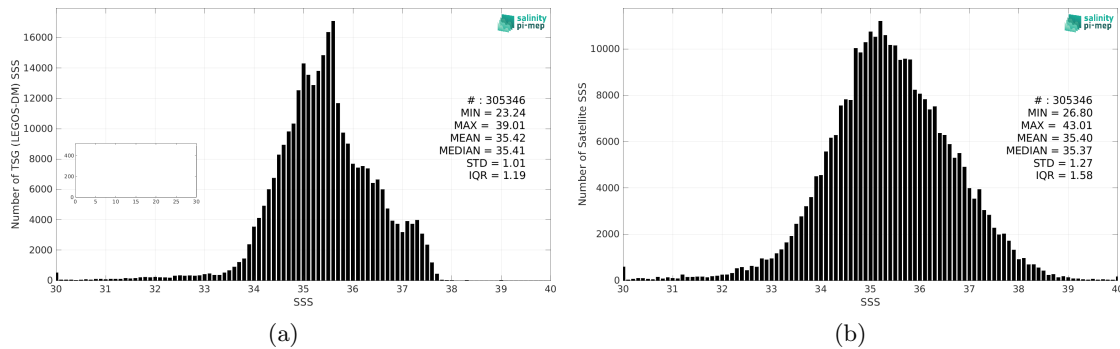
Figure 2: Histograms of SSS from TSG (LEGOS-DM) (a) and SMOS SSS L2Q v331 - 0.25 Deg (CATDS-CPDC) (b) considering all match-up pairs per bins of 0.1 over the Mid-Low Latitudes 45N-45S Pi-MEP region and for the full satellite product period.
