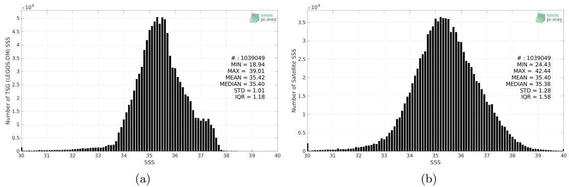
Figure 2: Histograms of SSS from TSG (LEGOS-DM) (a) and SMOS SSS L2Q v331 - 0.25 Deg (CATDS-CPDC) (b) considering all match-up pairs per bins of 0.1 over the Mid-Low Latitudes 45N-45S Pi-MEP region and for the full satellite product period.
