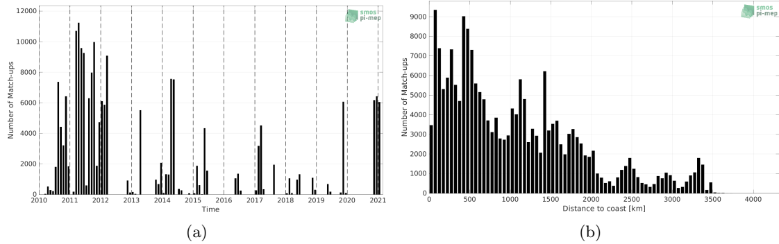
Figure 1: Number of match-ups between TSG (GOSUD-Sailing-ship) and SMOS SSS L2Q v331 - 0.25 Deg (CATDS-CPDC) SSS as a function of time (a) and as function of the distance to coast (b) over the Mid-Low Latitudes 45N-45S Pi-MEP region and for the full satellite product period.
