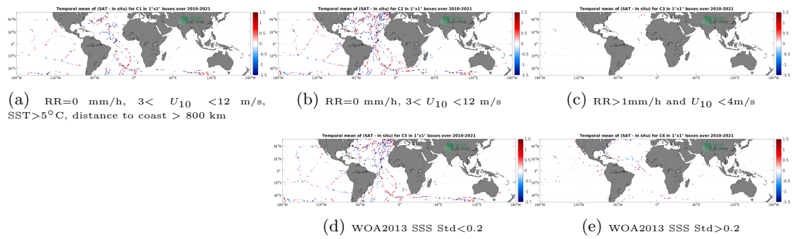
Figure 12: Temporal mean gridded over spatial boxes of size 1^\circ \times 1^\circ of \Delta SSS (SMOS SSS L2Q v331 - 0.25 Deg (CATDS-CPDC) - TSG (GOSUD-Sailing-ship)) for 5 different subdatasets corresponding to: RR=0 mm/h, 3 < U_{10} < 12 m/s, SST > 5°C, distance to coast > 800 km (a), RR=0 mm/h, 3 < U_{10} < 12 m/s (b), RR > 1mm/h and U_{10} < 4 m/s (c), WOA2013 SSS Std < 0.2 (d), WOA2013 SSS Std > 0.2 (e).
