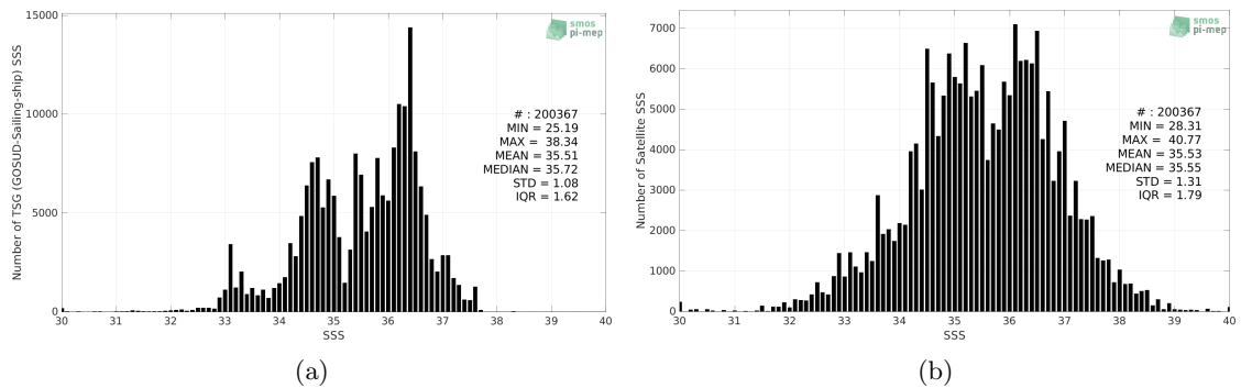
Figure 2: Histograms of SSS from TSG (GOSUD-Sailing-ship) (a) and SMOS SSS L2Q v331 - 0.25 Deg (CATDS-CPDC) (b) considering all match-up pairs per bins of 0.1 over the Mid-Low Latitudes 45N-45S Pi-MEP region and for the full satellite product period.
