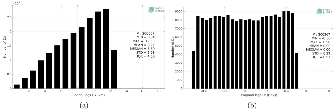
Figure 5: Histograms of the spatial (a) and temporal (b) lags between the location/time of the TSG (GOSUD-Sailing-ship) measurement and the date of the corresponding SMOS SSS L2Q v331 - 0.25 Deg (CATDS-CPDC) SSS pixel.
