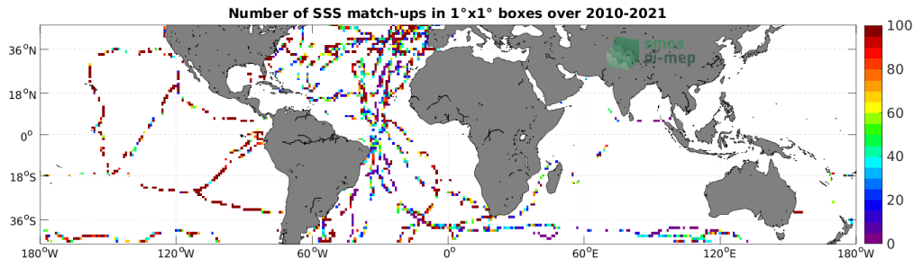
Figure 4: Number of SSS match-ups between TSG (GOSUD-Sailing-ship) SSS and the SMOS SSS L2Q v331 - 0.25 Deg (CATDS-CPDC) SSS product for the Mid-Low Latitudes 45N-45S Pi-MEP region over 1^\circ \times 1^\circ boxes and for the full satellite product period.
