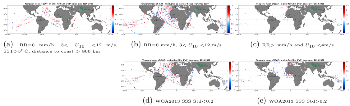
Figure 12: Temporal mean gridded over spatial boxes of size 1^\circ \times 1^\circ of \Delta\text{SSS} (SMOS SSS L2Q v331 - 0.25 Deg (CATDS-CPDC) - TSG (GOSUD-Research-vessel)) for 5 different subdatasets corresponding to: RR=0 mm/h, 3 < U_{10} < 12 m/s, SST > 5°C, distance to coast > 800 km (a), RR=0 mm/h, 3 < U_{10} < 12 m/s (b), RR > 1mm/h and U_{10} < 4 m/s (c), WOA2013 SSS Std < 0.2 (d), WOA2013 SSS Std > 0.2 (e).
