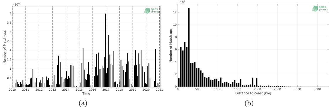
Figure 1: Number of match-ups between TSG (GOSUD-Research-vessel) and SMOS SSS L2Q v331 - 0.25 Deg (CATDS-CPDC) SSS as a function of time (a) and as function of the distance to coast (b) over the Mid-Low Latitudes 45N-45S Pi-MEP region and for the full satellite product period.
