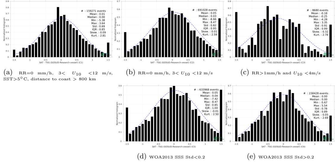
Figure 13: Normalized histogram of \Delta SSS (SMOS SSS L2Q v331 - 0.25 Deg (CATDS-CPDC) - TSG (GOSUD-Research-vessel)) for 5 different subdatasets corresponding to: RR=0 mm/h, 3 < U_{10} < 12 m/s, SST>5°C, distance to coast > 800 km (a), RR=0 mm/h, 3 < U_{10} < 12 m/s (b), RR>1mm/h and U_{10} < 4 m/s (c), WOA2013 SSS Std<0.2 (d), WOA2013 SSS Std>0.2 (e).
