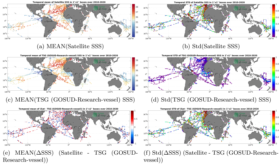
Figure 6: Temporal mean (left) and Std (right) of SSS from SMOS SSS L2Q v331 - 0.25 Deg (CATDS-CPDC) (top), TSG (GOSUD-Research-vessel) (middle), and of \Delta SSS (Satellite - TSG (GOSUD-Research-vessel)). Only match-up pairs are used to generate these maps.
