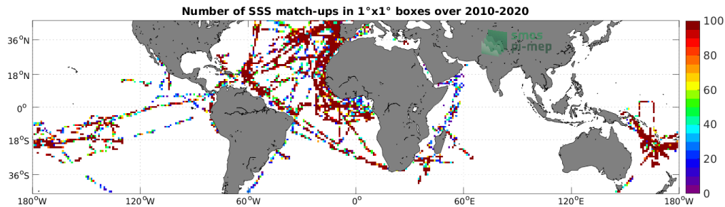
Figure 4: Number of SSS match-ups between TSG (GOSUD-Research-vessel) SSS and the SMOS SSS L2Q v331 - 0.25 Deg (CATDS-CPDC) SSS product for the Mid-Low Latitudes 45N-45S Pi-MEP region over 1^\circ \times 1^\circ boxes and for the full satellite product period.
