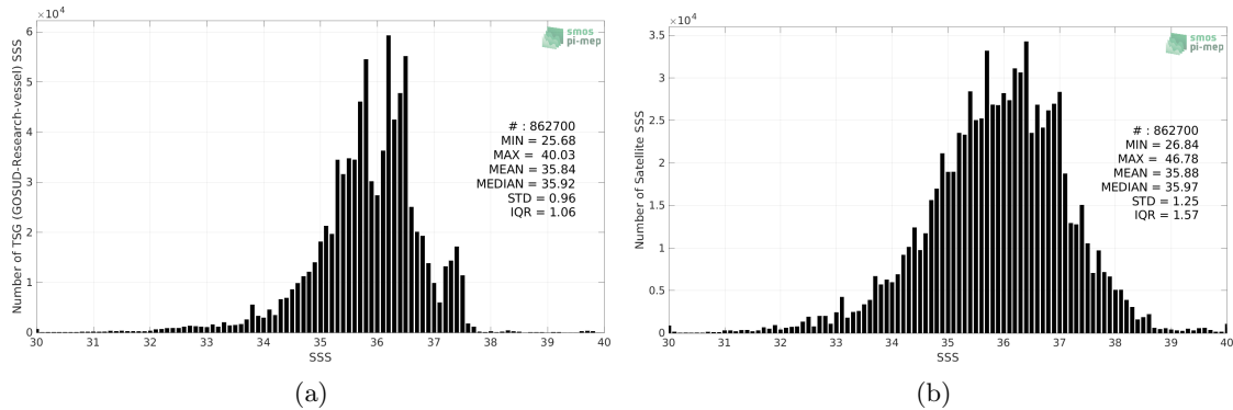
Figure 2: Histograms of SSS from TSG (GOSUD-Research-vessel) (a) and SMOS SSS L2Q v331 - 0.25 Deg (CATDS-CPDC) (b) considering all match-up pairs per bins of 0.1 over the Mid-Low Latitudes 45N-45S Pi-MEP region and for the full satellite product period.
