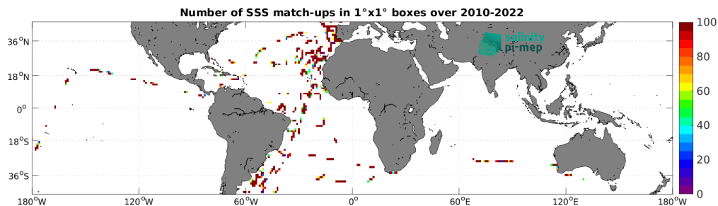
Figure 4: Number of SSS match-ups between TSG (CSIC-UTM) SSS and the SMOS SSS L2Q v331 - 0.25 Deg (CATDS-CPDC) SSS product for the Mid-Low Latitudes 45N-45S Pi-MEP region over 1^\circ \times 1^\circ boxes and for the full satellite product period.
