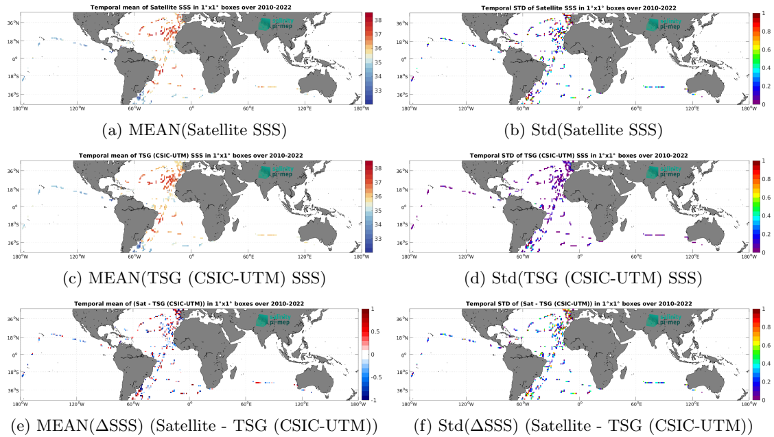
Figure 6: Temporal mean (left) and Std (right) of SSS from SMOS SSS L2Q v331 - 0.25 Deg (CATDS-CPDC) (top), TSG (CSIC-UTM) (middle), and of \Delta SSS (Satellite - TSG (CSIC-UTM)). Only match-up pairs are used to generate these maps.
