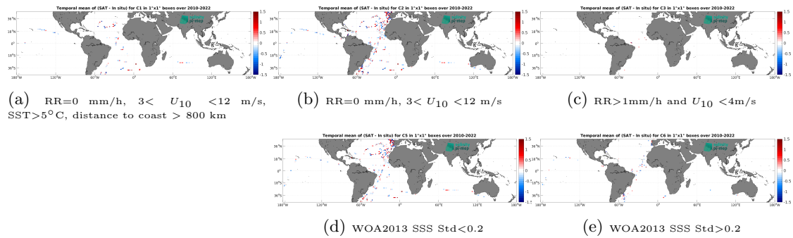
Figure 12: Temporal mean gridded over spatial boxes of size 1^\circ \times 1^\circ of \Delta SSS (SMOS SSS L2Q v331 - 0.25 Deg (CATDS-CPDC) - TSG (CSIC-UTM)) for 5 different subdatasets corresponding to:RR=0 mm/h, 3 < U_{10} < 12 m/s, SST >5^\circ\text{C} , distance to coast > 800 km (a), RR=0 mm/h, 3 < U_{10} < 12 m/s (b), RR >1 mm/h and U_{10} < 4 m/s (c), WOA2013 SSS Std <0.2 (d), WOA2013 SSS Std >0.2 (e).
