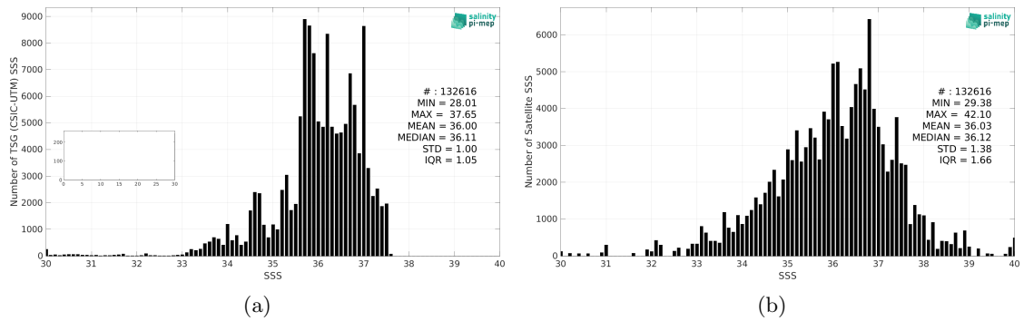
Figure 2: Histograms of SSS from TSG (CSIC-UTM) (a) and SMOS SSS L2Q v331 - 0.25 Deg (CATDS-CPDC) (b) considering all match-up pairs per bins of 0.1 over the Mid-Low Latitudes 45N-45S Pi-MEP region and for the full satellite product period.
