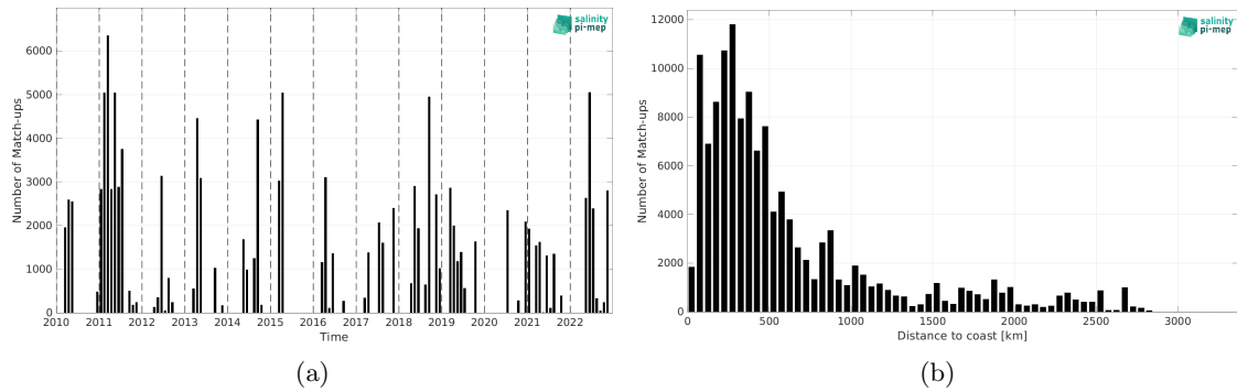
Figure 1: Number of match-ups between TSG (CSIC-UTM) and SMOS SSS L2Q v331 - 0.25 Deg (CATDS-CPDC) SSS as a function of time (a) and as function of the distance to coast (b) over the Mid-Low Latitudes 45N-45S Pi-MEP region and for the full satellite product period.
