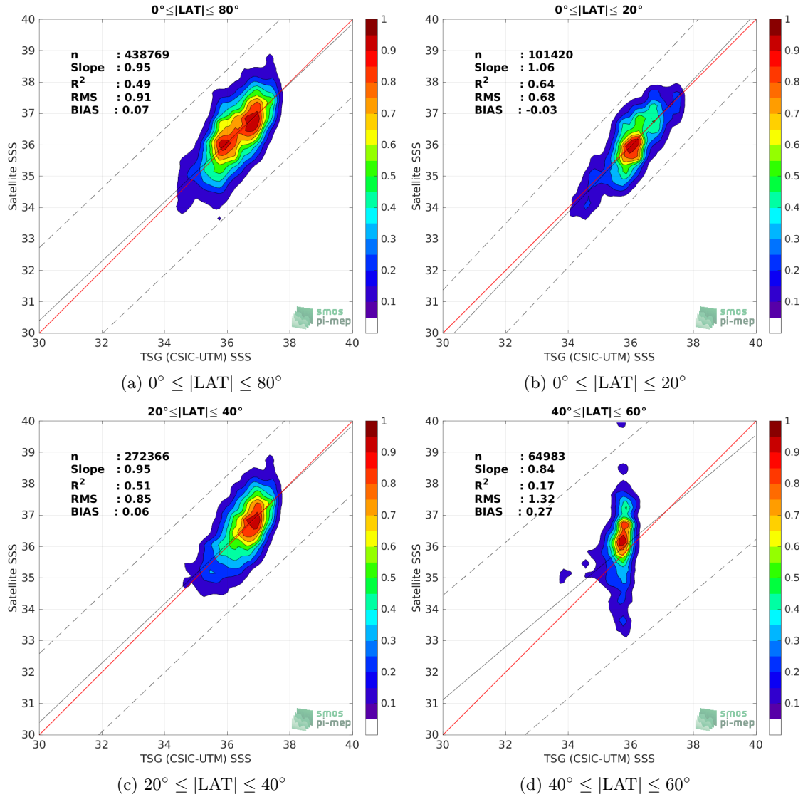
Figure 9: Contour maps of the concentration of SMOS SSS L2Q v331 - 0.25 Deg (CATDS-CPDC) SSS ( y -axis) versus TSG (CSIC-UTM) SSS ( x -axis) at match-up pairs for different latitude bands. For each plot, the red line shows x=y . The black thin and dashed lines indicate a linear fit through the data cloud and the \pm 95\% confidence levels, respectively. The number match-up pairs n , the slope and R^2 coefficient of the linear fit, the root mean square (RMS) and the mean bias between satellite and in situ data are indicated for each latitude band in each plots.
