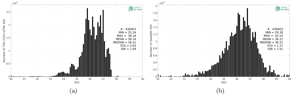
Figure 2: Histograms of SSS from TSG (CSIC-UTM) (a) and SMOS SSS L2Q v331 - 0.25 Deg (CATDS-CPDC) (b) considering all match-up pairs per bins of 0.1 over the Mid-Low Latitudes 45N-45S Pi-MEP region and for the full satellite product period.
