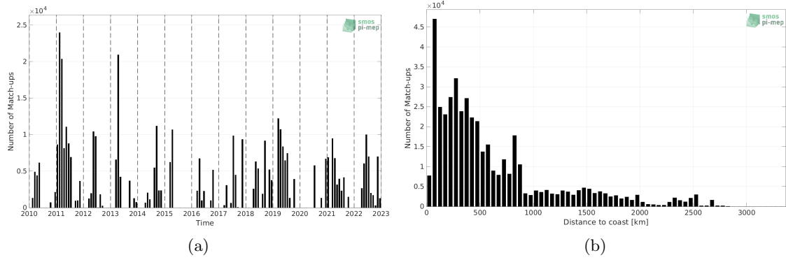
Figure 1: Number of match-ups between TSG (CSIC-UTM) and SMOS SSS L2Q v331 - 0.25 Deg (CATDS-CPDC) SSS as a function of time (a) and as function of the distance to coast (b) over the Mid-Low Latitudes 45N-45S Pi-MEP region and for the full satellite product period.
