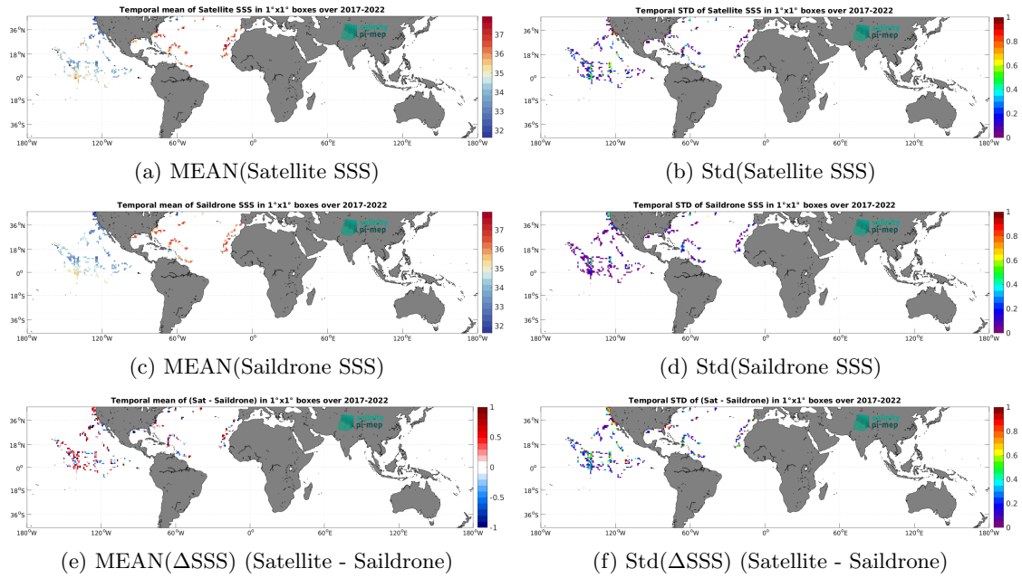
Figure 6: Temporal mean (left) and Std (right) of SSS from SMOS SSS L2Q v331 - 0.25 Deg (CATDS-CPDC) (top), Saildrone (middle), and of \Delta SSS (Satellite - Saildrone). Only match-up pairs are used to generate these maps.
