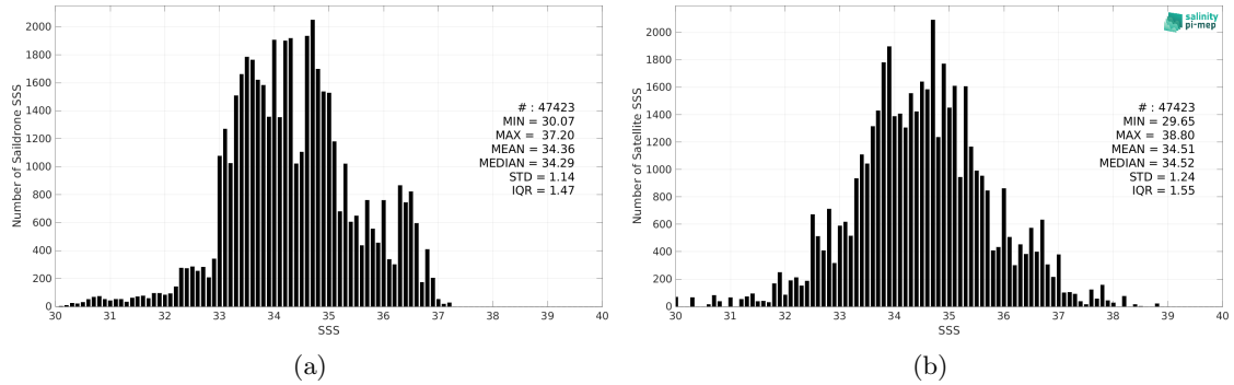
Figure 2: Histograms of SSS from Saildrone (a) and SMOS SSS L2Q v331 - 0.25 Deg (CATDS-CPDC) (b) considering all match-up pairs per bins of 0.1 over the Mid-Low Latitudes 45N-45S Pi-MEP region and for the full satellite product period.
