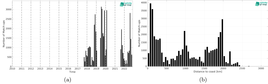
Figure 1: Number of match-ups between Saildrone and SMOS SSS L2Q v331 - 0.25 Deg (CATDS-CPDC) SSS as a function of time (a) and as function of the distance to coast (b) over the Mid-Low Latitudes 45N-45S Pi-MEP region and for the full satellite product period.
