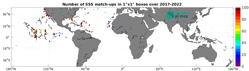
Figure 4: Number of SSS match-ups between Saildrone SSS and the SMOS SSS L2Q v331 - 0.25 Deg (CATDS-CPDC) SSS product for the Mid-Low Latitudes 45N-45S Pi-MEP region over 1^\circ \times 1^\circ boxes and for the full satellite product period.
