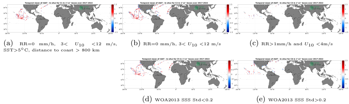
Figure 12: Temporal mean gridded over spatial boxes of size 1^\circ \times 1^\circ of \Delta SSS (SMOS SSS L2Q v331 - 0.25 Deg (CATDS-CPDC) - Saildrone) for 5 different subdatasets corresponding to: RR=0 mm/h, 3 < U_{10} < 12 m/s, SST > 5^\circ\text{C} , distance to coast > 800 km (a), RR=0 mm/h, 3 < U_{10} < 12 m/s (b), RR > 1 mm/h and U_{10} < 4 m/s (c), WOA2013 SSS Std < 0.2 (d), WOA2013 SSS Std > 0.2 (e).
