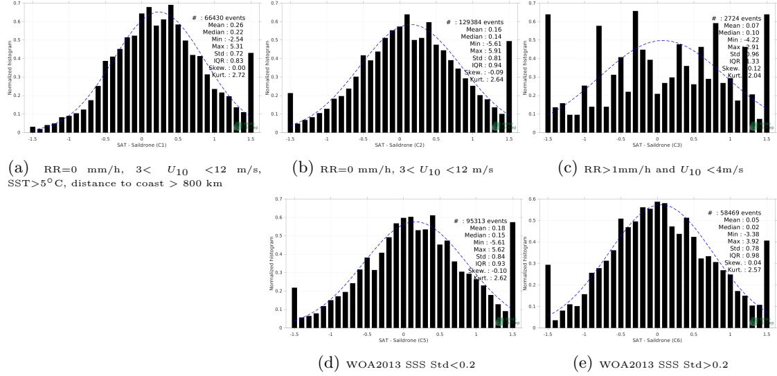
Figure 13: Normalized histogram of \Delta SSS (SMOS SSS L2Q v331 - 0.25 Deg (CATDS-CPDC) - Sairdrone) for 5 different subdatasets corresponding to: RR=0 mm/h, 3 < U_{10} < 12 m/s, SST>5°C, distance to coast > 800 km (a), RR=0 mm/h, 3 < U_{10} < 12 m/s (b), RR>1mm/h and U_{10} < 4 m/s (c), WOA2013 SSS Std<0.2 (d), WOA2013 SSS Std>0.2 (e).
