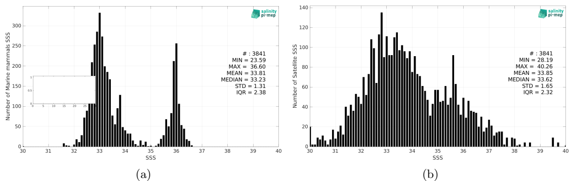
Figure 2: Histograms of SSS from Marine mammals (a) and SMOS SSS L2Q v331 - 0.25 Deg (CATDS-CPDC) (b) considering all match-up pairs per bins of 0.1 over the Mid-Low Latitudes 45N-45S Pi-MEP region and for the full satellite product period.
