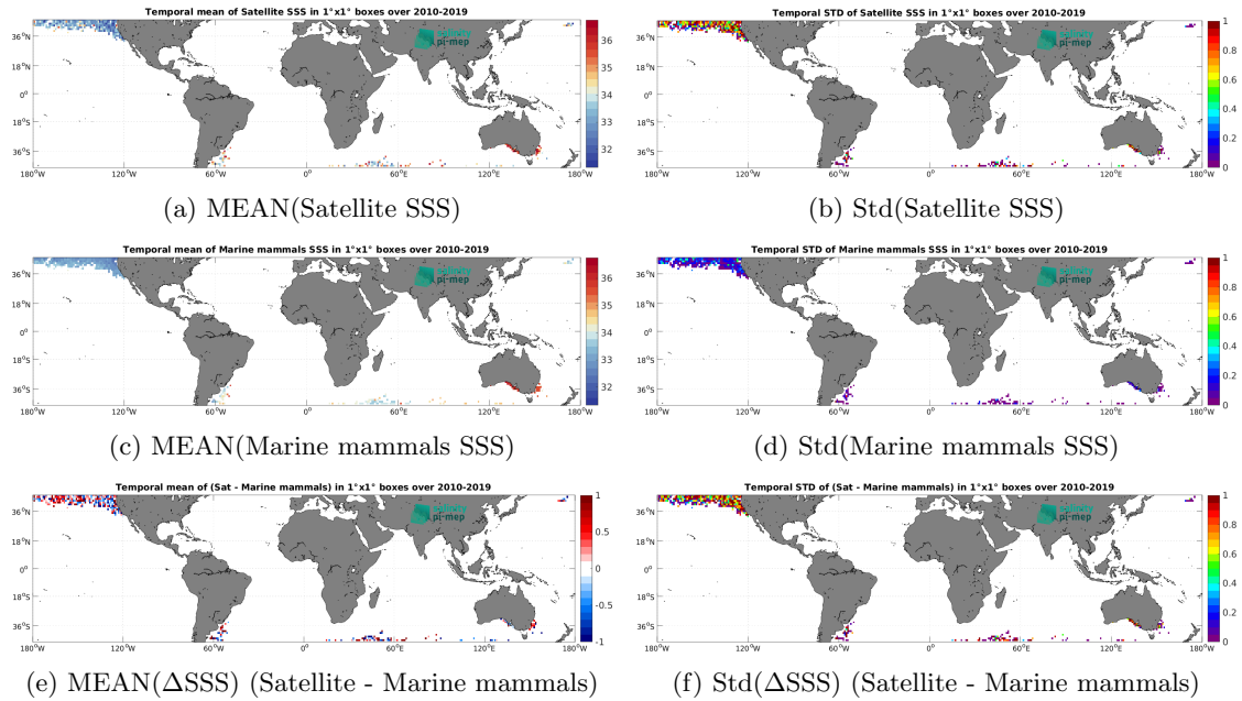
Figure 6: Temporal mean (left) and Std (right) of SSS from SMOS SSS L2Q v331 - 0.25 Deg (CATDS-CPDC) (top), Marine mammals (middle), and of \Delta SSS (Satellite - Marine mammals). Only match-up pairs are used to generate these maps.
