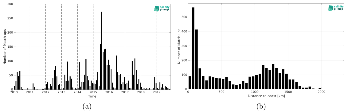
Figure 1: Number of match-ups between Marine mammals and SMOS SSS L2Q v331 - 0.25 Deg (CATDS-CPDC) SSS as a function of time (a) and as function of the distance to coast (b) over the Mid-Low Latitudes 45N-45S Pi-MEP region and for the full satellite product period.
