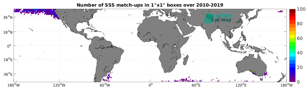
Figure 4: Number of SSS match-ups between Marine mammals SSS and the SMOS SSS L2Q v331 - 0.25 Deg (CATDS-CPDC) SSS product for the Mid-Low Latitudes 45N-45S Pi-MEP region over 1^\circ \times 1^\circ boxes and for the full satellite product period.
