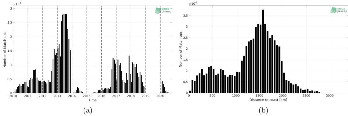
Figure 1: Number of match-ups between Surface drifters and SMOS SSS L2Q v331 - 0.25 Deg (CATDS-CPDC) SSS as a function of time (a) and as function of the distance to coast (b) over the Mid-Low Latitudes 45N-45S Pi-MEP region and for the full satellite product period.
