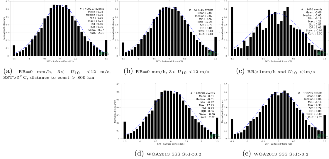
Figure 12: Normalized histogram of \Delta SSS (SMOS SSS L2Q v331 - 0.25 Deg (CATDS-CPDC) - Surface drifters) for 5 different subdatasets corresponding to: RR=0 mm/h, 3 < U_{10} < 12 m/s, SST>5°C, distance to coast > 800 km (a), RR=0 mm/h, 3 < U_{10} < 12 m/s (b), RR>1mm/h and U_{10} < 4 m/s (c), WOA2013 SSS Std<0.2 (d), WOA2013 SSS Std>0.2 (e).
