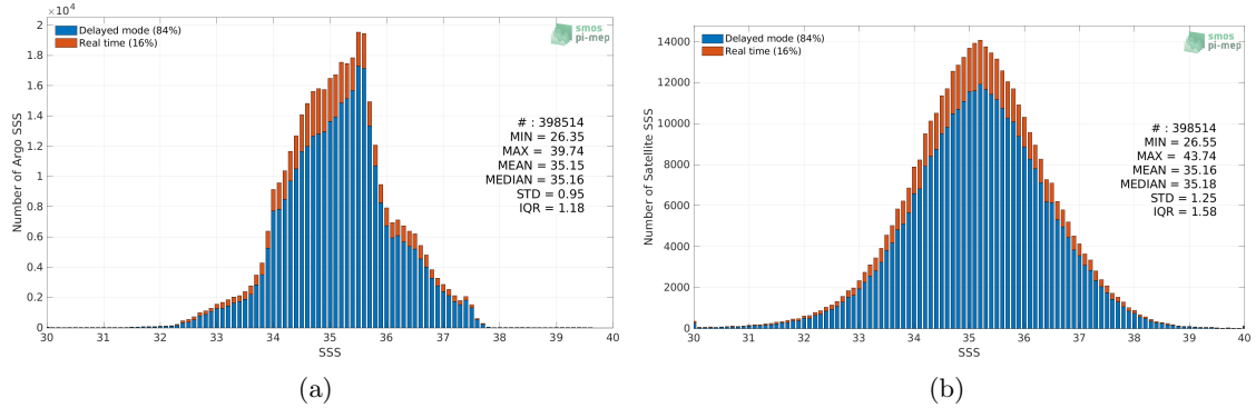
Figure 2: Histograms of SSS from Argo (a) and SMOS SSS L2Q v331 - 0.25 Deg (CATDS-CPDC) (b) considering all match-up pairs per bins of 0.1 over the Mid-Low Latitudes 45N-45S Pi-MEP region and for the full satellite product period.
