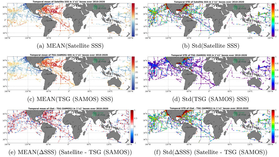
Figure 6: Temporal mean (left) and Std (right) of SSS from SMOS SSS L2Q v330 - 0.25 Deg (CATDS-CPDC) (top), TSG (SAMOS) (middle), and of \Delta SSS (Satellite - TSG (SAMOS)). Only match-up pairs are used to generate these maps.
