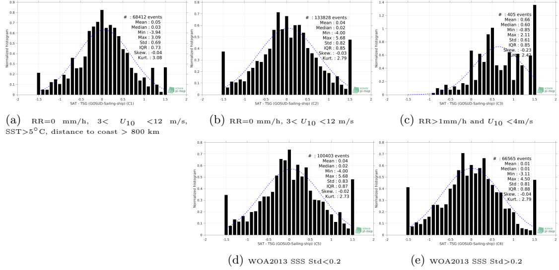
Figure 13: Normalized histogram of \Delta SSS (SMOS SSS L2Q v330 - 0.25 Deg (CATDS-CPDC) - TSG (GOSUD-Sailing-ship)) for 5 different subdatasets corresponding to: RR=0 mm/h, 3 < U_{10} < 12 m/s, SST>5°C, distance to coast > 800 km (a), RR=0 mm/h, 3 < U_{10} < 12 m/s (b), RR>1mm/h and U_{10} < 4 m/s (c), WOA2013 SSS Std<0.2 (d), WOA2013 SSS Std>0.2 (e).
