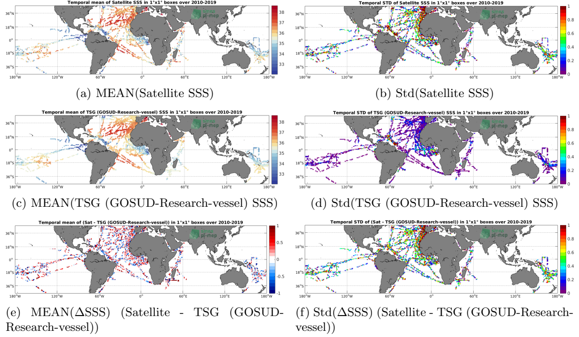
Figure 6: Temporal mean (left) and Std (right) of SSS from SMOS SSS L2Q v330 - 0.25 Deg (CATDS-CPDC) (top), TSG (GOSUD-Research-vessel) (middle), and of \Delta SSS (Satellite - TSG (GOSUD-Research-vessel)). Only match-up pairs are used to generate these maps.
