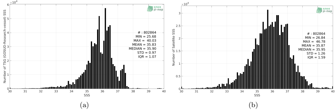
Figure 2: Histograms of SSS from TSG (GOSUD-Research-vessel) (a) and SMOS SSS L2Q v330 - 0.25 Deg (CATDS-CPDC) (b) considering all match-up pairs per bins of 0.1 over the Mid-Low Latitudes 45N-45S Pi-MEP region and for the full satellite product period.
