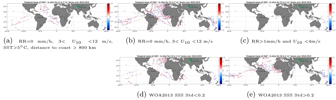
Figure 12: Temporal mean gridded over spatial boxes of size 1^\circ \times 1^\circ of \Delta SSS (SMOS SSS L2Q v330 - 0.25 Deg (CATDS-CPDC) - TSG (GOSUD-Research-vessel)) for 5 different subdatasets corresponding to: RR=0 mm/h, 3 < U_{10} < 12 m/s, SST > 5^\circ C , distance to coast > 800 km (a), RR=0 mm/h, 3 < U_{10} < 12 m/s (b), RR > 1 mm/h and U_{10} < 4 m/s (c), WOA2013 SSS Std < 0.2 (d), WOA2013 SSS Std > 0.2 (e).
