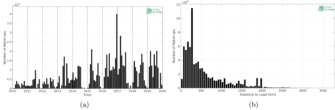
Figure 1: Number of match-ups between TSG (GOSUD-Research-vessel) and SMOS SSS L2Q v330 - 0.25 Deg (CATDS-CPDC) SSS as a function of time (a) and as function of the distance to coast (b) over the Mid-Low Latitudes 45N-45S Pi-MEP region and for the full satellite product period.
