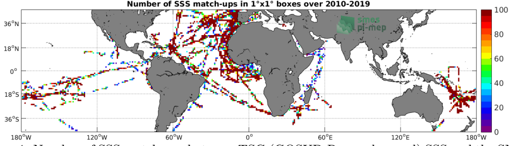
Figure 4: Number of SSS match-ups between TSG (GOSUD-Research-vessel) SSS and the SMOS SSS L2Q v330 - 0.25 Deg (CATDS-CPDC) SSS product for the Mid-Low Latitudes 45N-45S Pi-MEP region over 1^\circ \times 1^\circ boxes and for the full satellite product period.
